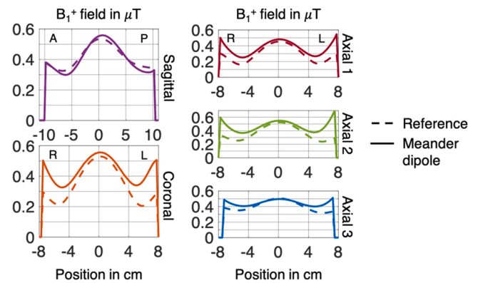
Fig. 5. Numerically B_1^+ profiles of the head coil alone (dashed lines) and with the meander dipoles (in solid lines) for each of the chosen slices.
