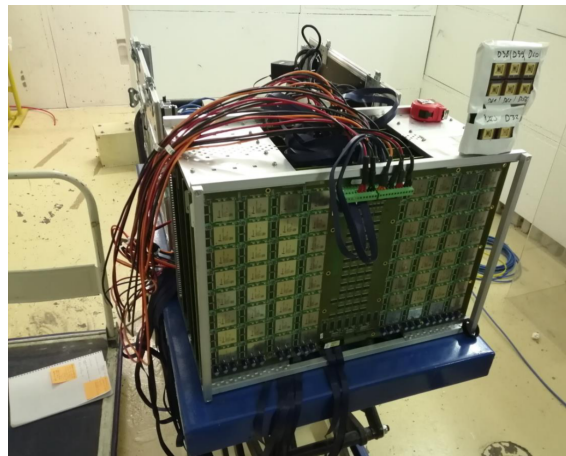
Fig. 1. Detail of the real-time soft-error rate testbench showing the measurement rack with 384 SRAM circuits in vertical position at GENESIS facility during the 14 MeV neutron irradiation campaign.
