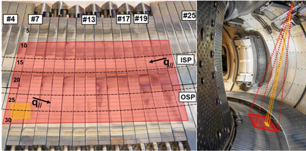
Figure 3 Left panel: focus on the 14 ITER-like PFUs of the WEST test divertor sector. PFUs monitored by the VHR IR camera are shown in the red areas from PFU #6 to PFU #21. Orange area represents the field of view (FoV) monitored by the VHR IR camera on PFU #7 and #8, discussed in this work. MBs are labeled from MB1, high field side (HFS), to MB35, low field side (LFS), as indicated in the PFU #6. Black arrows indicate the parallel heat flux direction in inner (HFS) and outer (LFS) divertor. Right panel: tangential view of the WEST vacuum vessel showing the VHR IR FoV (orange) and the potential position that can be observed with the VHR (red).
