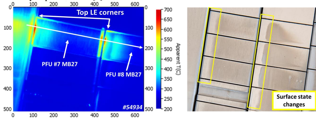
Figure 4 Left panel: IR thermography on shot #54934 monitoring PFU#7 (chamfered) and #8 (sharp) at the OSP (MB27). Right panel: picture of the same FoV taken after the C4 experimental campaign that evidences the surface states changes. The FoV shows a top view of the WEST divertor, whose PFUs run along the poloidal direction.
