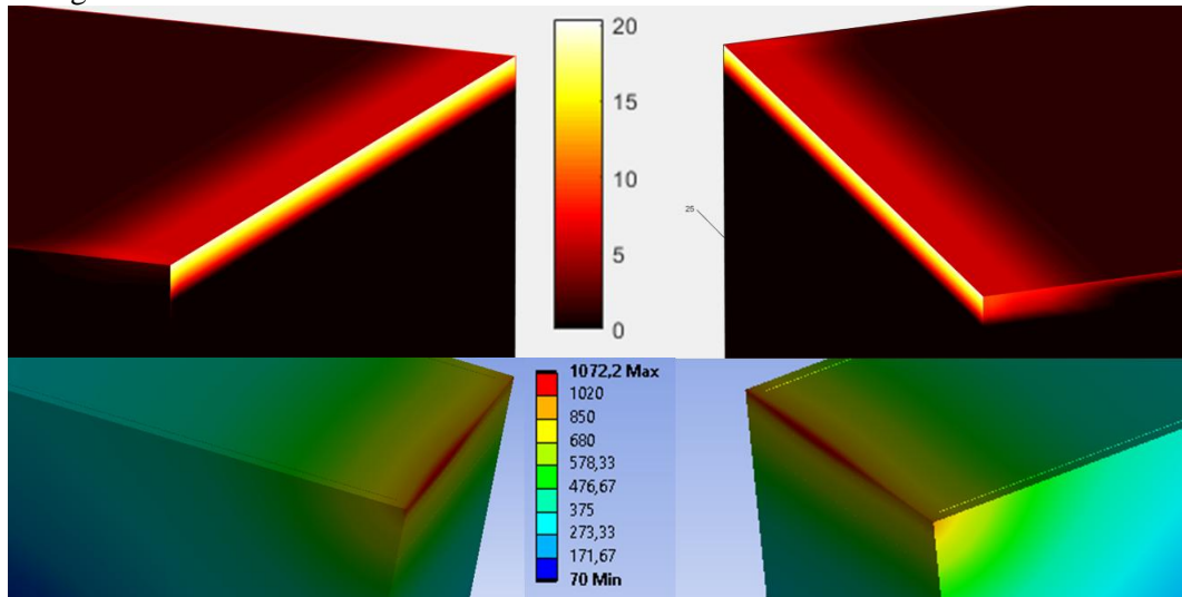
Figure 11 Top panel: normalized ( 1 \text{ MW.m}^{-2} on top surface far from the LE) 3D particle distribution using ion orbit modeling on a misaligned LE of PFU#8 MB27 (0.4 mm). The simulation considers the shadowing induced by the neighboring PFUs ([25]). Focus on the top LE corner in the toroidal gap between MB26 and MB27 (left), and bottom LE corner in the toroidal gap between MB27 and MB28 (right). Bottom panel: 3D FEM thermal modeling analogous to Figure 9, with IO modeling.
