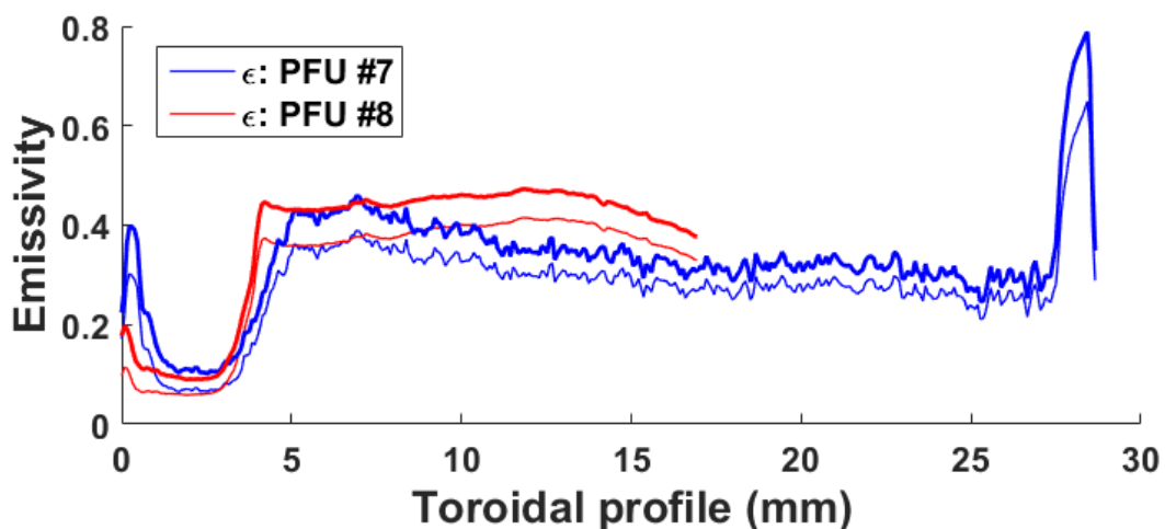
Figure 7 Toroidal profiles of emissivity, measured at 50°C (thin curves) and extrapolated to the MB temperature (thick curves) for PFU #7 (blue), #8 (red).
