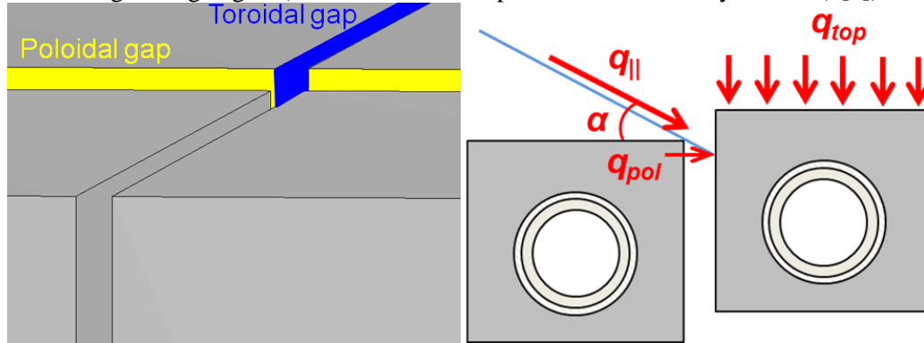
Figure 1 Left panel: poloidal gaps (yellow) between two PFUs, and toroidal gaps (blue) between two monoblocks of the same PFU. Right panel: magnetic field line impinging the poloidal side of the misaligned monoblock (blue line) with a parallel heat flux coming from the scrape-off layer ( q_{||} ) and an incidence angle ( \alpha ). Heat flux absorbed on the top surface ( q_{top} ), and on the side surface ( q_{pol} ) are also depicted on the misaligned MB. In case of misalignment, the exposed area is larger on the poloidal side.
