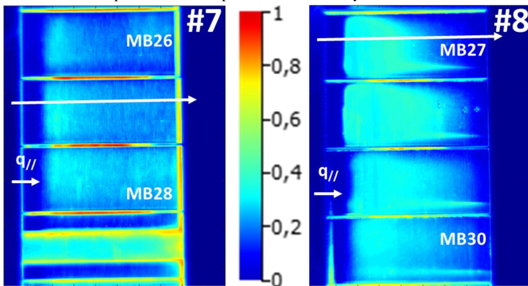
Figure 6 Emissivity measurement performed at 50^{\circ}\text{C} and atmospheric pressure on ITER-like PFUs after the C4 experimental campaign at the OSP: chamfered PFU #7 (left), sharp PFU #8 (right).
