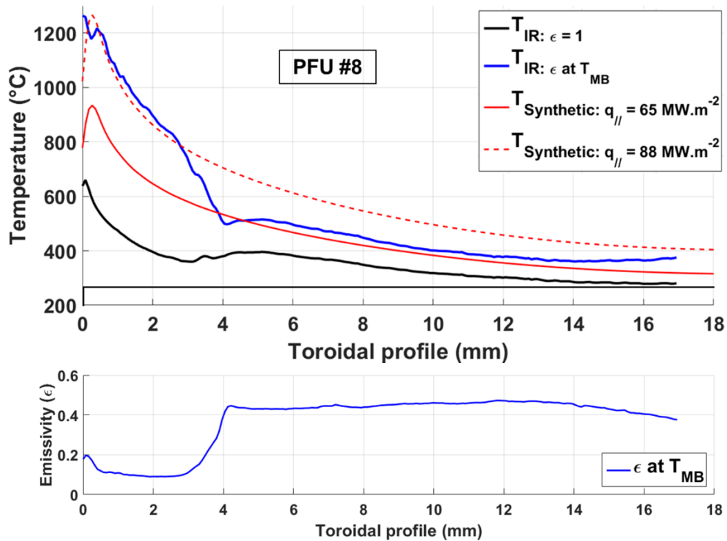
Figure 8 Top panel: Comparison between IR temperatures corrected with non-uniform emissivity (blue) with synthetic data obtained through 3D FEM modeling in a toroidal profile of PFU #8 MB27 on shot #54934. The dash-red line ( q_{||} = 88 \text{ MW.m}^{-2} ) matches with the IR LE temperature while the full red line ( 65 \text{ MW.m}^{-2} ) matches with the top surface, far from the LE. The black line represents the black-body temperature. Bottom panel: emissivity extrapolated to the real temperature of the MB along the toroidal profile.
