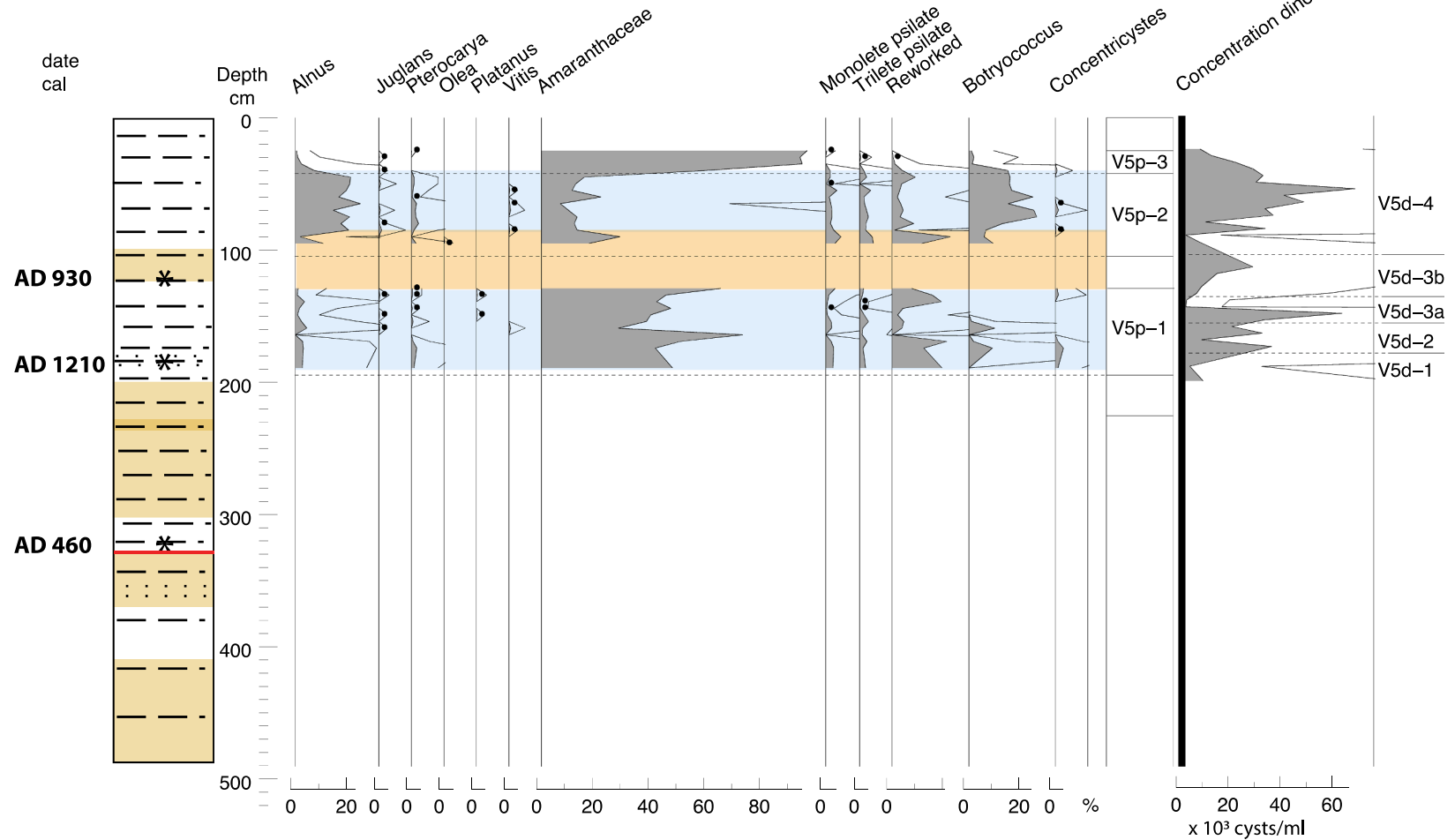
Fig. 5. Selected curves pollen and dinocysts of core V5 (full diagrams in SI) with magnetic susceptibility. Dates shown (*) are the cal AD/BC median probability of the radiocarbon calibrated age range.
