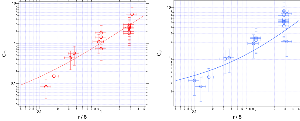
Figure 4: Dimensionless drag mass and friction coefficients determined as C_m = \frac{m^* \omega}{2\pi\eta} and C_\beta = \frac{\beta^*}{2\pi\eta} as a function of r/\delta for liquids of different viscosities and densities (listed in Table 2). The solid lines correspond to the theoretical values of C_m and C_\beta from the model. See text for details.
