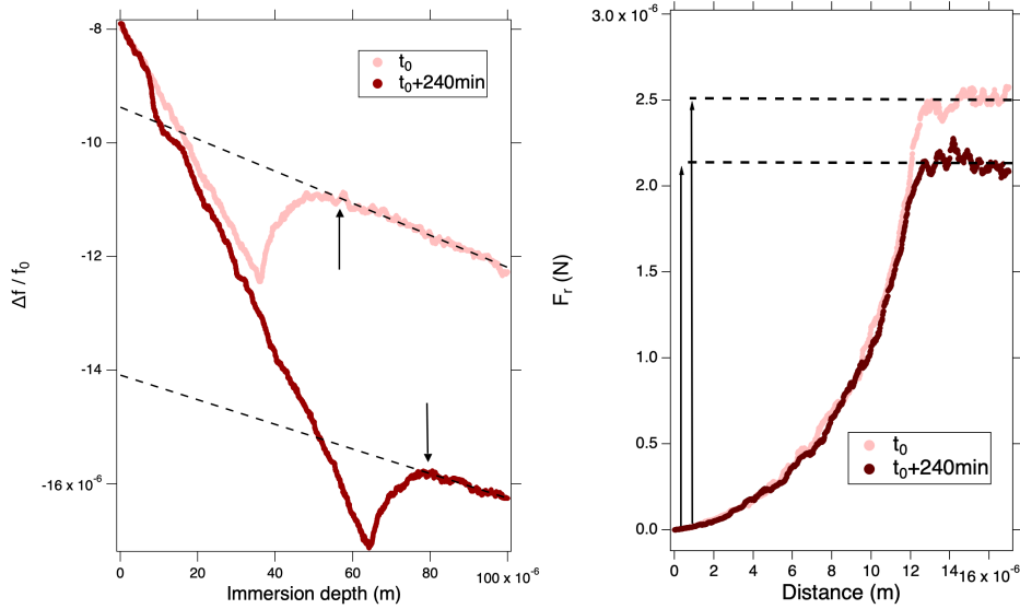
Figure 8: Plot of the frequency shift (left) and meniscus rupture force (right) at the PDMS water interface at t_0 and t_0+240\text{min} during upward motion of the oscillating fiber. The point where the water meniscus is pinned at the apex of the fiber is marked by arrows. The breaking force is proportional interfacial tension. To calculate it, the dragged mass contribution (linear fit plotted as dashed lines) to the frequency shift is first subtracted from the data. Based on F_r values, and a fiber radius r = 6.5\mu\text{m} , interfacial tension \gamma = 53.4(\pm 3.9)\text{mN}\cdot\text{m}^{-1} at t_0 , and \gamma = 37.5(\pm 3.5)\text{mN}\cdot\text{m}^{-1} at t_0 + 240\text{min}
