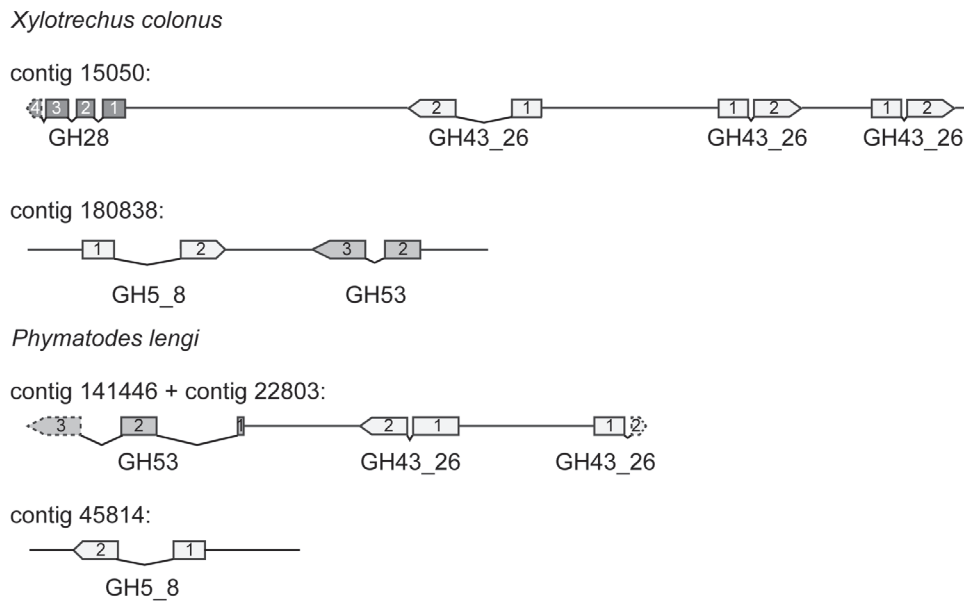
Fig. 4. Structure and organization of genes encoding PCWDEs in Xylotrechus colonus and Phymatodes lengi . Short read datasets corresponding to shallow genome sequencing projects of the two Cerambycinae species X. colonus and P. lengi were retrieved from GenBank and assembled. Selected contigs containing genes encoding representatives of several PCWDE families are depicted for X. colonus and P. lengi . Exons are indicated by boxes in various shades of grey for each gene. Dashed boxes indicate that a portion of the sequence is missing. Individual exons are numbered for each gene.
