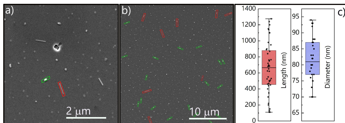
Figure 3: SEM images of the surface after deposition of 4.5 ML Mn on Ge(111) wafer and annealing at 650^\circ\text{C} for 15 min at (a) higher and (b) lower magnification. The two populations of 3D islands can be clearly distinguished with several small round islands and some long and short NWs. c) Length and diameter distribution of the NWs. The whiskers define minimum and maximum value of each dimension, while the boxes show the 25th and 75th percentile of the distribution with the middle line representing the average value of \approx 700 \text{ nm} for the length and \approx 80 \text{ nm} for the diameter.
