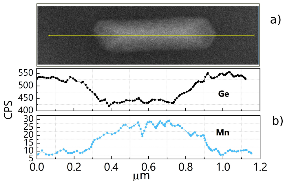
Figure 4: (a) SEM image of a typical NW, \approx 700 \text{ nm} long, obtained by deposition of a 4.5 ML thick Mn film followed by annealing at 650^\circ\text{C} for 15 min. (b) Mn and Ge EDX line profiles along the yellow line drawn in (a).
