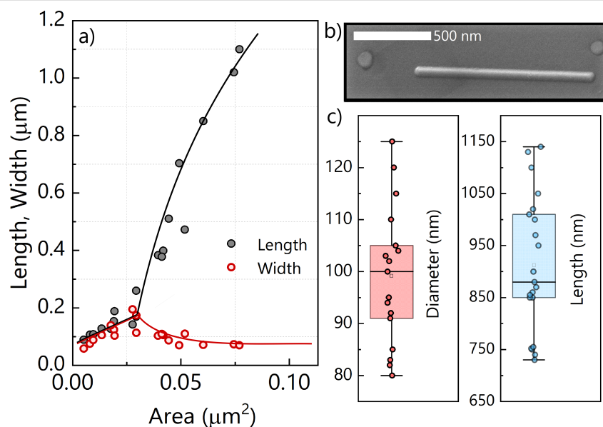
Figure 7: (a) Length ( t ) and width ( s ) of \text{Mn}_5\text{Ge}_3 islands, formed on the sample surface of the 4.5 ML thick Mn layer upon annealing at 650 °C for 15 min, as functions of the island area. Deviation from a regular island shape (diverging branches) occurs at s = t \approx 170 nm. At area values of \approx 0.075 \mu\text{m}^2 , the width approaches the optimal value of s = 80 nm (red line) while the length continues to grow (black line). Lines are guides to the eyes. (b) SEM image of the typical morphology of a NW (after annealing for 30 min at 650 °C) to facilitate the comparison with experiment. (c) Diameter and length distribution of NWs (conditions similar to that in (b)). The whiskers show the minimum and maximum value of NW dimensions, while the colored boxes show the 25th and 75th percentile of the distribution with the middle line representing the average value.
