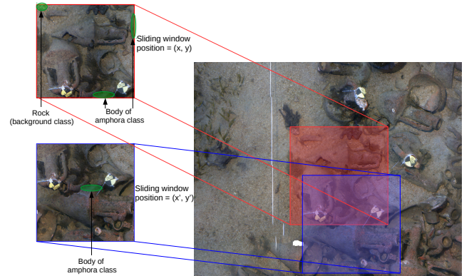
Fig. 2. Representation of the content of the sliding window at two different positions. The red sliding window shows two pieces of amphora on the border and one piece of rock which can not be identified by human. The blue sliding window represents the same amphora as the red one but it can be easily identified using the entire content.
