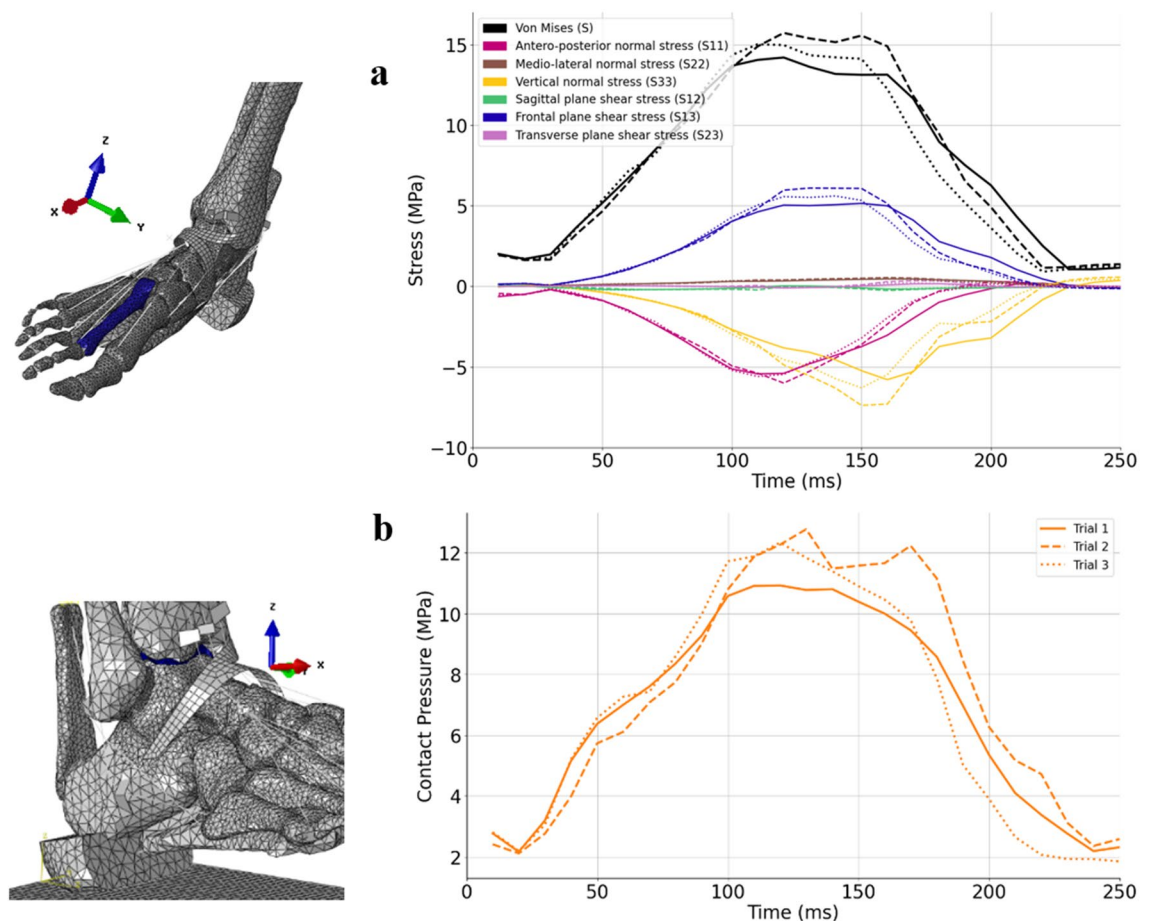
Figure 5. (a) Average of Von Mises stresses (in black) and of the stress tensor components (in color) on the second metatarsal for the three trials during the stance phase. S11(magenta), S22 (brown), and S33 (yellow) are respectively the normal stresses in anteroposterior (x-axis), mediolateral (y-axis), and vertical (z-axis) directions. S12 (green), S13 (blue), and S23 (purple) are respectively the shear stresses in sagittal, frontal, and transverse planes. (b) Average of the contact pressure undergone by the tibiotalar cartilage. For both graphs, each trial is represented by a different line style (1 = solid, 2 = dashed & 3 = dotted).
