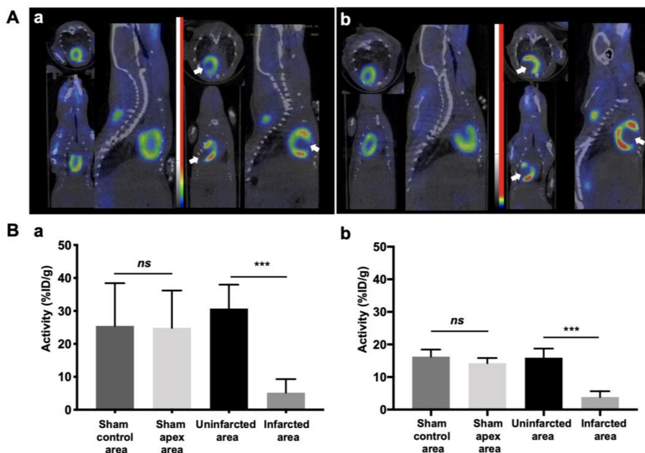
Figure 2. Myocardial infarction resulted in myocardial viability defect evaluated by ^{18}\text{F} -FDG microPET imaging. (A) ^{18}\text{F} -FDG microPET imaging showed a signal decrease in the infarcted myocardium identified by a white arrow at day 16 (a) and at day 30 (b) post-surgery. (B) Semi-quantitative analysis expressed as percentage of injected dose per gram of mouse (%ID/g mean \pm SD) for day 16 (a) to day 30 (b) post-surgery showed a significant decreased in Apex area compared to control area (Mean apex = 5.19 \pm 4.10\% ID/g, Mean control = 30.7 \pm 7.25\% ID/g, n = 7 ; *** p = 0.0003 at day 16) and (Mean apex = 3.84 \pm 1.81\% ID/g, Mean control = 15.9 \pm 2.81\% ID/g, n = 7 ; *** p = 0.0003 at day 30). In contrast, uptake was homogeneous in sham hearts for both experiment time (Mean apex = 24.8 \pm 11.3\% ID/g, Mean control = 25.4 \pm 12.9\% ID/g, n = 4 ; ns: p = 0.443 at day 16) and (Mean apex , 14.3 \pm 1.54\% ID/g, Mean control 16.2 \pm 2.20\% ID/g, n = 4 ; ns: p = 0.885 at day 30).
