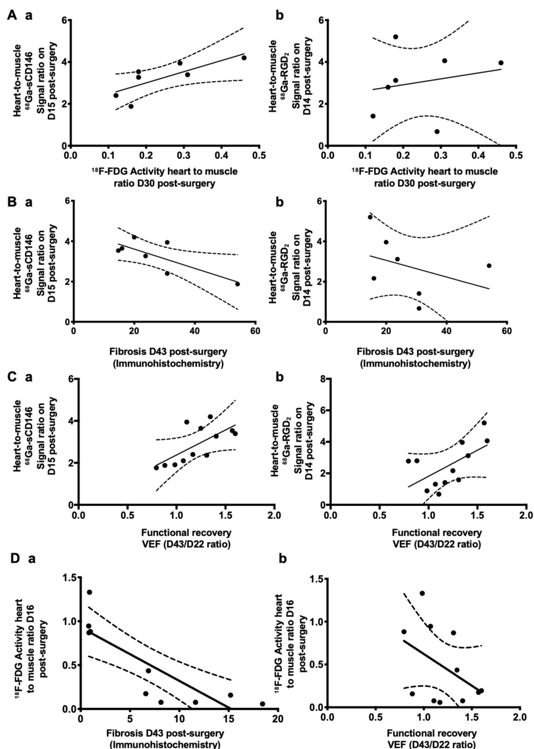
Figure 5. Correlation analysis. (Aa) Significant positive correlation between residual perfusion recovery evaluated by ^{18}\text{F-FDG} microPET signal expressed as heart-to-muscle ratio on day 30 and ^{68}\text{Ga-sCD146} microPET signal intensity expressed as heart-to-muscle ratio on day 15 post-myocardial infarction (Pearson R^2 = 0.70 ; p = 0.04 ; n = 7 ). (Ab) No significant correlation was observed between individual residual perfusion recovery and ^{68}\text{Ga-RGD}_2 microPET signal intensity on day 14 post-ischemia (Pearson R^2 = 0.21 ; p = 0.64 ; n = 7 ). (Ba): Significant negative correlation was detected between individual fibrosis quantification evaluated by histological Sirius red staining and
