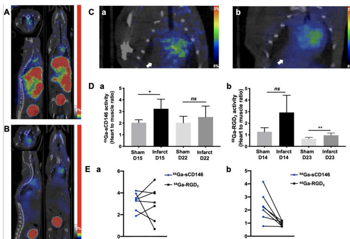
Figure 4. AMOT expression evaluated by ^{68}\text{Ga} -sCD146 microPET imaging was early increased after myocardial infarction. (A) Representative whole body PET images of ^{68}\text{Ga} -sCD146 on infarcted heart. (B) Representative whole body PET images of ^{68}\text{Ga} -RGD 2 on infarcted heart and PET imaging on infarcted heart. (C) Representative cardiac-focused images of ^{68}\text{Ga} -sCD146 (a) and ^{68}\text{Ga} -RGD 2 (b) PET imaging on infarcted heart. White arrow indicates the infarcted myocardium area. (D) Semi-quantitative analysis of ^{68}\text{Ga} -sCD146 PET uptake (a) expressed as heart-to-muscle ratio, showed an early and significant increase in infarcted hearts at day 15 compared to sham hearts ( H/M_{\text{ischemic}} = 3.23 \pm 0.82 , n = 7 , H/M_{\text{sham}} = 2.03 \pm 0.25 , n = 4 ; * p = 0.04 ) and a trend of increasing uptake at day 22 post-surgery ( H/M_{\text{ischemic}} = 2.52 \pm 0.94 , n = 7 ; H/M_{\text{sham}} = 2.02 \pm 0.56 , n = 4 ; ns: p = 0.30 ). Semi-quantitative analysis of ^{68}\text{Ga} -RGD 2 PET uptake (b), expressed as heart-to-muscle ratio, showed a delayed but significant increase in the infarcted heart compared to sham hearts at day 23 post-surgery ( H/M_{\text{ischemic}} = 0.96 \pm 0.18 , n = 7 , H/M_{\text{sham}} = 0.65 \pm 0.12 , n = 4 ; p = 0.02 ). No uptake modification was observed before this time ( H/M_{\text{ischemic}} = 2.92 \pm 1.48 ; H/M_{\text{sham}} = 1.26 \pm 0.13 , n = 7 , ns: p = 0.15 at day 14 post-myocardial infarction). (E) Semi-quantitative intra-animal comparison of both tracers, ^{68}\text{Ga} -sCD146 and ^{68}\text{Ga} -RGD 2 at early times, respectively D14 and D15 after MI surgery (a). No significant difference was observed between ^{68}\text{Ga} -sCD146 and ^{68}\text{Ga} -RGD 2 PET uptake in the infarcted heart at this time ( n = 7 ; p = 0.93 ). Semi-quantitative intra-animal comparison was also realized a later time, respectively D22 and D23 for ^{68}\text{Ga} -sCD146 and ^{68}\text{Ga} -RGD 2 (b). A significant difference was observed between ^{68}\text{Ga} -sCD146 and ^{68}\text{Ga} -RGD 2 PET uptakes in the infarcted hearts at this later time ( n = 7 ; ** p = 0.01 ).
