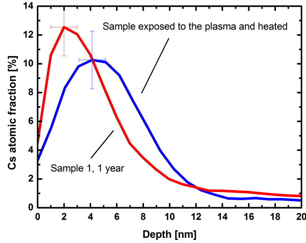
Figure 5. Comparison of the depth profiles from the sample 1 (never exposed to the plasma) and the sample used during the plasma campaign.
