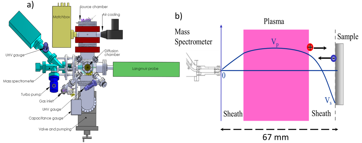
Figure 2. a) Sketch of the ECR reactor test bed [41], b) sample-mass spectrometer arrangement, V_s and V_p are the sample and plasma potential respectively.
