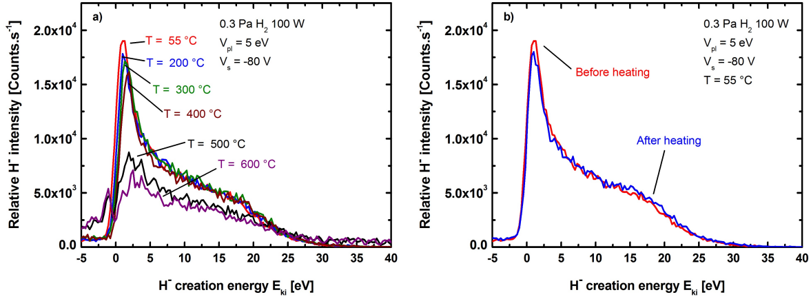
Figure 4. a): H - creation energy for a sample temperature of 55 °C, 200 °C, 300 °C, 400 °C, 500 °C, 600 °C and for a 0.3 Pa H 2 , 100 W plasma and -80 V sample bias, b): H - creation energy for a sample temperature of 55 °C obtained before heating and after cooling phase.
