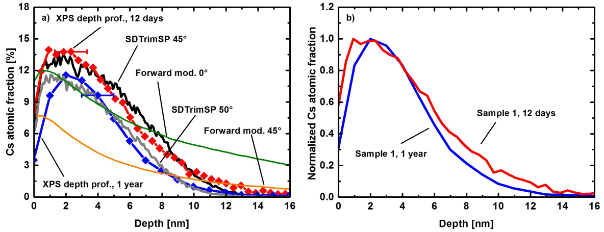
Figure 1. a) Caesium atomic fraction for: XPS depth profiling performed twelve days and one year after implantation, the SDTrimSP simulation for 45^\circ and 50^\circ incidence angles, the forward modelling for 0^\circ and 45^\circ incidence angles, b) normalization of the experimental curves of fig 1a).
