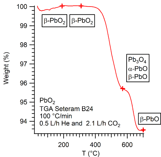
Figure 2: TGA curve of the thermal decomposition of plattnerite in \text{CO}_2 . Insets indicate the products that were identified by \mu -XRD.
