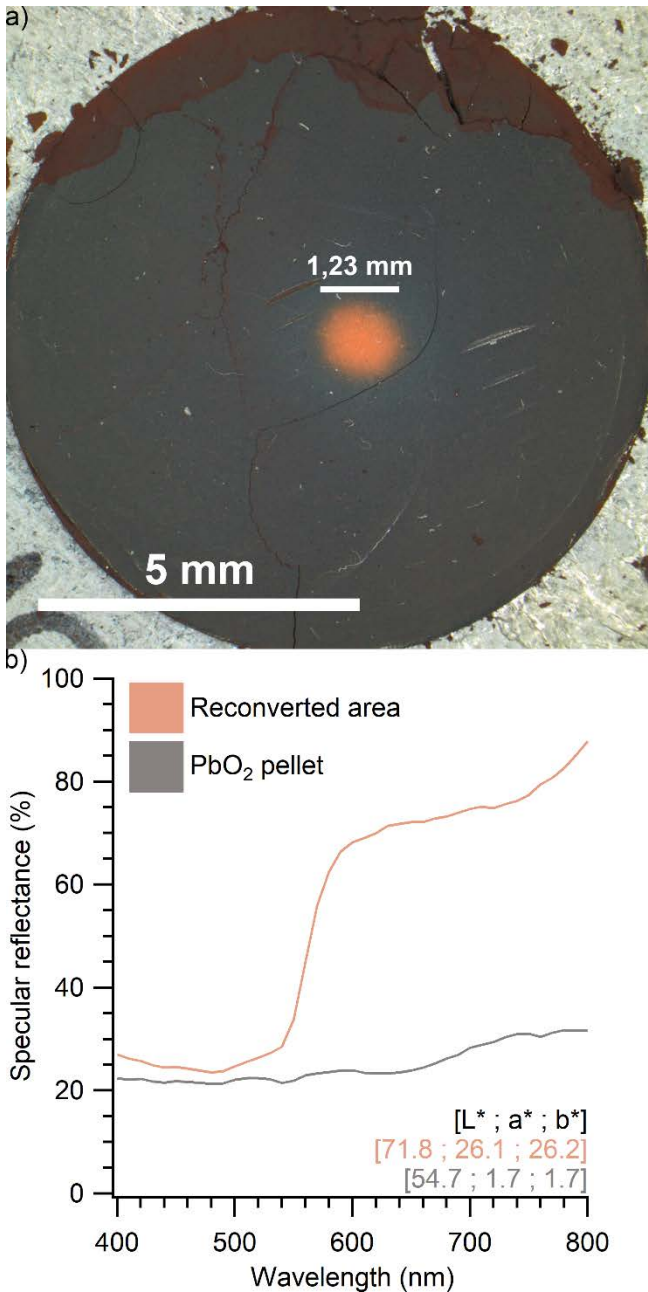
Figure 4a) Pure 440 \mu\text{m} -thick plattnerite pellet that has been exposed to a 3.48 mm diameter 1080 nm diode laser beam ( 1/e value) at a 205 \text{ kW m}^{-2} irradiance during 2 min. b) specular reflectance spectra of the irradiated and pristine areas of the same pellet. Colour patches have been displayed using the RGB values calculated from the L^*a^*b^* coordinates.
