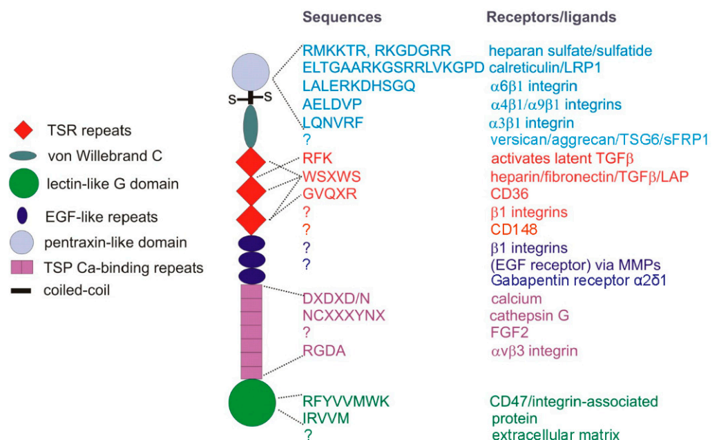
Figure 1. TSP1 subunit domains and their cell surface receptors or extracellular ligands. TSP1 is a ~450 kDa homotrimer of subunits linked by disulfide bonds near the N-terminal pentraxin-like domain. Type 1 TSP1 repeats (TSR), EGF-like, and calcium-binding repeats form the central stalk region of TSP1, connecting the N- and C-terminal globular domains.
