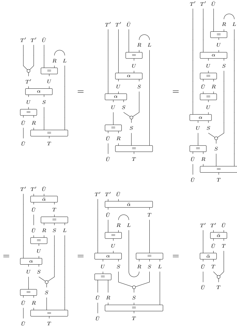
Figure 1: Proof of \bar{\alpha} \circ (\mu^T \bar{U}) = (\bar{U} \mu^S) \circ (\bar{\alpha} T) \circ (T' \bar{\alpha}) .
