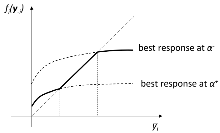
Figure 3: Non linear best response with loss aversion
