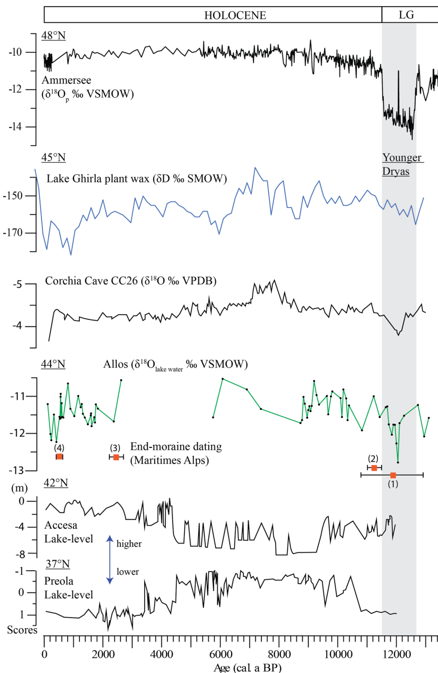
Figure 6. Estimated \delta^{18}\text{O} ( \delta^{18}\text{O}_{\text{lw}} , ‰ VSMOW) in the lake waters of Lake Allos compared to other records: oxygen isotope ratios in precipitation ( \delta^{18}\text{O}_p , ‰ VSMOW) based on the record of Lake Ammersee (Germany; von Grafenstein et al. , 1999); Lake Ghirla plant wax ( \delta D , ‰ SMOW) at the foot of the Southern Alps (Wirth and Sessions, 2016); oxygen isotope record ( \delta^{18}\text{O} , ‰ VPDB) of Corchia Cave CC26 (Northern Italy; Zanchetta et al. , 2007); lake-level fluctuations (m) at Accesa (Italy; Magny et al. , 2007); lake level reconstruction at Preola (Southern Italy; Magny et al. , 2011). Locations of the sites are shown on Fig. 1. Ages of end-moraine and polished bedrock (Maritime Alps) dated by ^{10}\text{Be} and ^{14}\text{C} methods are from: (1) Spagnolo and Ribolini (2019); (2) Darnault et al. (2012); (3) Federici et al. (2008); (4) Ribolini et al. (2007); and (5) Federici and Stefanini (2001). [Color figure can be viewed at wileyonlinelibrary.com ]
