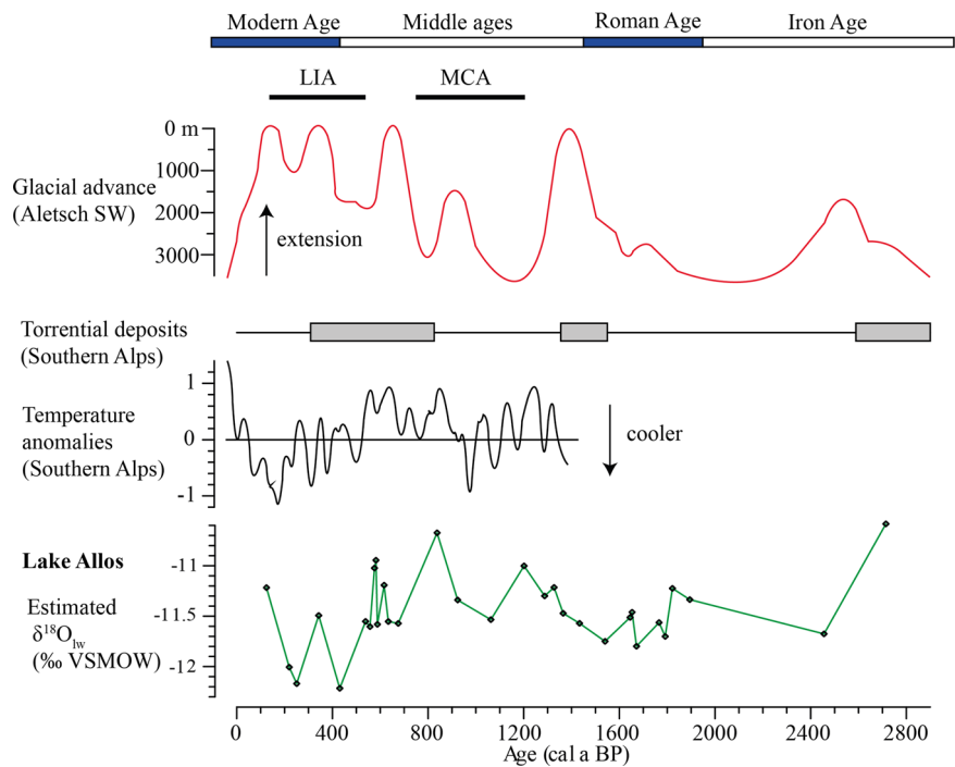
Figure 7. Estimated \delta^{18}\text{O} ( \delta^{18}\text{O}_{\text{lw}} , ‰ VSMOW) in Allos' lake waters for the last 3000 years compared to global signatures of the Medieval Climate Anomaly (MCA) and Little Ice Age (LIA) (Mann et al. , 2009), glacial advances at Aletsch in Switzerland (Holzhauser et al. , 2005), torrential deposits in Southern French Alps (Sivan et al. , 2006) and temperature anomalies reconstructed from dendrochronological data (Corona et al. , 2011). [Color figure can be viewed at wileyonlinelibrary.com ]
