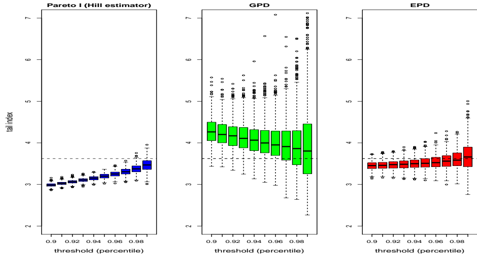
Figure 2: Boxplots of maximum likelihood estimators of the tail index: 1,000 samples of 50,000 observations drawn from a Singh-Maddala distribution, SM(2.07, 1.14, 1.75) . From the left to the right, the x -axis is the threshold (percentile) used to fit Pareto I (blue), GPD (green) and EPD (red) models.
