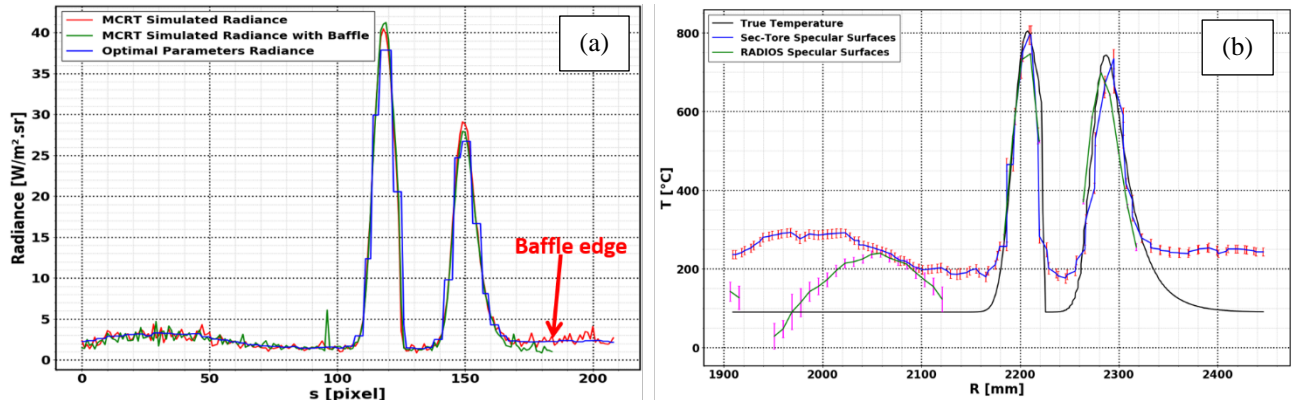
Figure 9 – (a): Synthetic noisy measurements (radiance profiles) built with the MCRT code in the case of specular reflective surfaces without baffle (red) and with baffle (green). Comparison with the optimal radiance profile obtained with the temperature estimated by the inverse method Sec-Tore (blue). (b): 3D temperature profile estimated with Sec-Tore (blue) with the associated levels of confidence and with RADIO5 (green) in the case of synthetic measurements with specular reflective surfaces. Profiles correspond to the green lines drawn on the 3D view of Figure 7, the origin being on the inner side.
