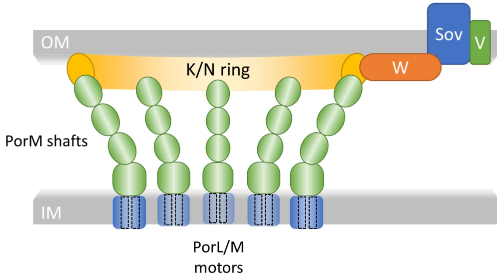
Figure 1: Multiple PorL/M motors form a funnel-shaped cage in the periplasm
