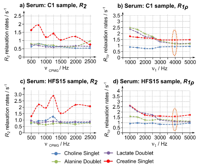
Figure 2. R_2 and R_{1\rho} relaxation rates as a function of \nu_{CPMG} and \nu_1 respectively for C and HFS serum samples relative to peaks of four metabolites. (a) R_2 and (b) R_{1\rho} for the C1 sample, (c) R_2 and (d) R_{1\rho} for the HFS15 sample. Dotted lines are used to help visually track the progress of R_{1\rho} .
