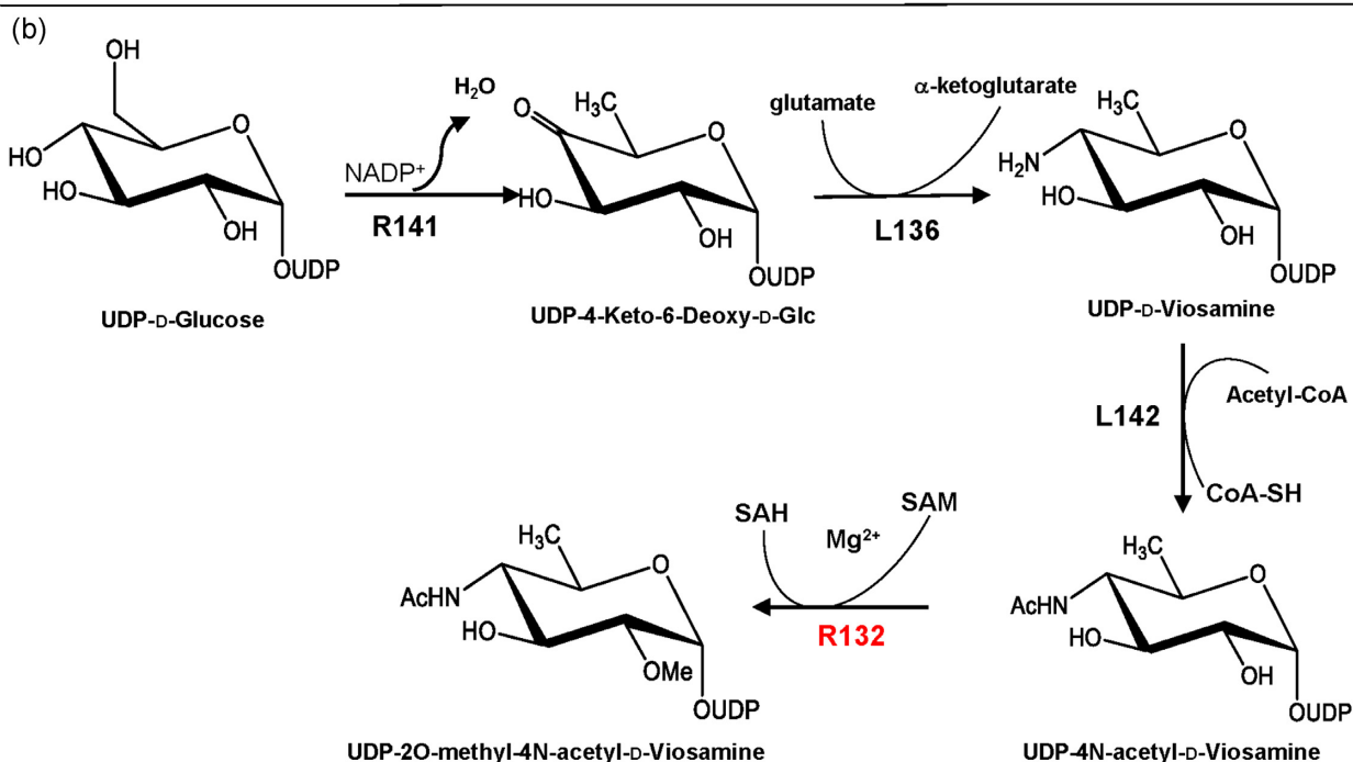
Figure 4. R132 methyltransferase, a candidate for viosamine methylation. (a) Multiple alignment of the C-Ter of MycE (PDB 3SSN), R132 of Mimivirus (YP_003 986 624), its homolog in Mamavirus (AEQ60310.1), Hirudovirus strain Sangsue (AHA45742.1) and Mimivirus Bombay (AMZ02580.1). The blue rectangles indicate the residues involved in catalytic activity: the two aspartates coordinating the magnesium D275 and D304 (Akey et al. 2011) are conserved in R132 and A-clade (D127 and D156); the histidine residue (H278) involved in deprotonation of the 2-OH is also conserved (H138). (b) Proposed biosynthetic pathway for the UDP-D-2O-methyl-4N-acetyl-viosamine. The functions of the first three enzymes have been experimentally validated and R132, based on in silico analysis, would be the missing methyltransferase.
