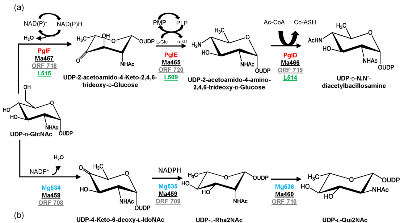
Figure 5. Proposed Moumouvirus australiensis (a) UDP-D-diNacBac pathway shared with Tupanviruses and (b) UDP-L-Qui2NAc synthetic pathway shared with Cotonvirus japonicus . Campylobacter jejuni proteins (Pgl, red) are used as reference for the bacillosamine pathway and Megavirus chilensis proteins (Mg, blue) for the quinovosamine pathway. The corresponding Moumouvirus australiensis (Ma, black), Cotonvirus japonicus (ORF, dark gray) and Tupanvirus deep ocean (L, light green) proteins are underlined. The NCBI accession number of protein sequences, their lengths and functions are reported in Table 1.
