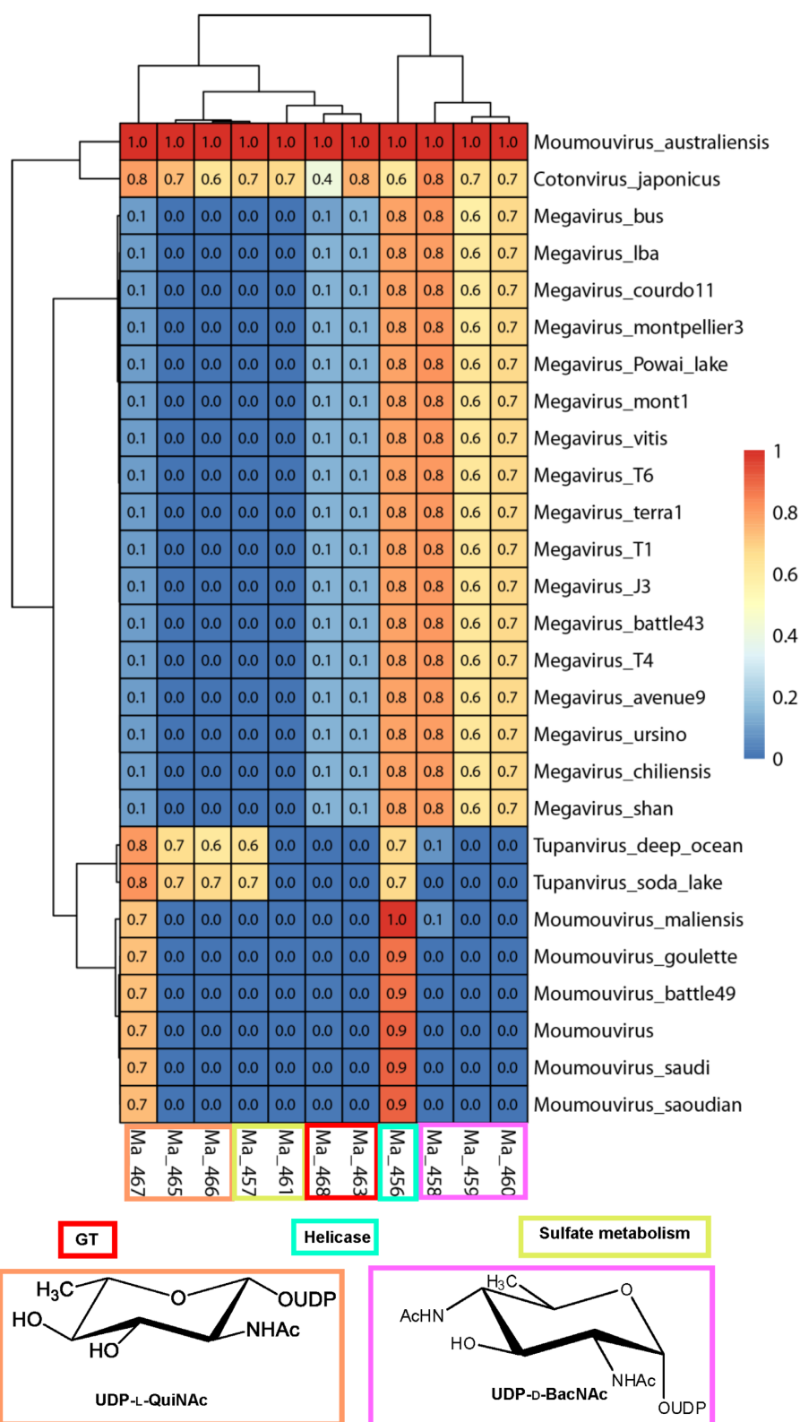
Figure 11. Heatmap of the conservation level of the Moumouvirus australiensis 12-glycogene cluster in the B-clade, C-clade, D-clade ( Tupanviruses ) and E-clade ( Cotonvirus japonicus ). Proteins involved in the UDP-L-QuiNAc and UDP-D-BacNAc biosynthetic pathways are in orange and pink, respectively. The GTs are in red, while proteins responsible for sulfate metabolism are in dark yellow. The helicase Ma456 (in cyan) is used for reference of the conservation level between clades. The two papain-like proteins (Ma462, Ma464) are not included because they are not directly related to fibrils glycosylation. The conservation score for each protein in the different genomes ranges from 0 to 1 (low to high: blue to red).
