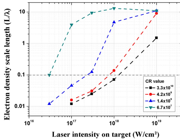
Figure 2. Simulated pre-plasma density scale length L normalized by \lambda for the four experimental CR studied and from I = 3.0 \times 10^{16} \text{ W/cm}^2 to 1.0 \times 10^{19} \text{ W/cm}^2 . At relativistic laser intensity regime ( I > 2.2 \times 10^{18} \text{ W/cm}^2 ), the Lorentz factor \gamma must be considered in the calculation of the critical density n_c , giving a measured L at I = 10^{19} \text{ W/cm}^2 lower than the one at I = 10^{18} \text{ W/cm}^2 for \text{CR} = 6.7 \times 10^7 . The grey horizontal dashed line represents L/\lambda = 0.1 .
