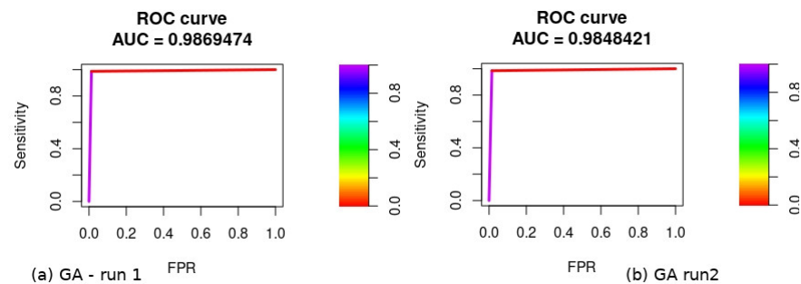
Figure 11. ROC curve for the validation set. Model performance was evaluated using the receiver operating characteristic (ROC) curve. The area under the curve is denoted AUC. The AUC obtained was 0.9869 for the first run with the genetic algorithm and 0.9848 for the second run. A large area under the curve was observed for both models. These models could then determine whether a variant was benign or pathogenic with a minimal error rate.
