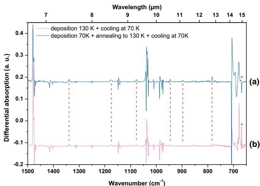
Figure 7. Comparison of the subtraction spectrum (after-before UV irradiation experiments) for both cases 1 and 2 benzene ice deposition conditions: (a) deposition 70 K followed by an annealing to 130 K and then cooling at 70 K (case 1) (b) deposition at 130 K followed by a cooling down to 70 K (case 2); *CO 2 (g): dashed lines photo-produced absorption bands common to both experiments.
