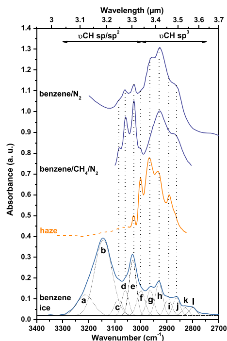
Figure 9. Deconvolved infrared spectrum of irradiated benzene ice residue (bottom, blue line) produced by photochemistry ( \lambda > 230 nm) and subsequently warmed up to room temperature compared with VIMS solar occultation spectrum at 203 km altitude (Bellucci et al., 2009; Kim et al., 2011) (orange solid line, processed by Carrasco et al. [2018] from Kim et al. [2011] between 3,050 and 2,825 \text{cm}^{-1} ), and orange dashed line corresponds to Titan's haze spectra from Kim et al. [2011] above 3,050 \text{cm}^{-1} ). The experimental spectrum is also compared with the IR spectra of aerosols generated from a \text{N}_2:\text{C}_6\text{H}_6 gas mixture submitted to UV irradiation (Gautier et al., 2017) (top, blue) or from a \text{N}_2:\text{CH}_4:\text{C}_6\text{H}_6 gas mixture in a cold plasma discharge (Sciamma-O'Brien et al., 2017). For the interpretation of the legend, the reader must refer to the web version of this article.
