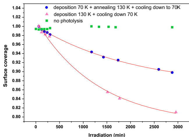
Figure 5. Evolution of the surface coverage of the benzene \nu_2 + \nu_{13} + \nu_{18} combination mode at 70 K for nonirradiated ice (squares), and during irradiation for ice deposited at 70 K, annealed to 130 K and cooling down to 70 K (circles, case 1) and ice deposited at 130 K and cooled to 70 K (triangles, case 2). The decrease is fitted by a single exponential decay.
