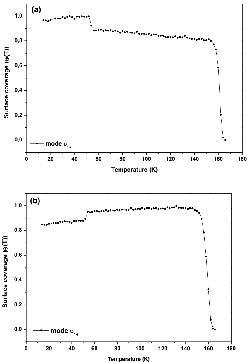
Figure 2. Surface coverage of C_6H_6 \nu_{13} (a) and \nu_{14} (b) modes as function of temperature ( 1.2\text{ K}\cdot\text{min}^{-1} ) determined by FTIR spectroscopy.
