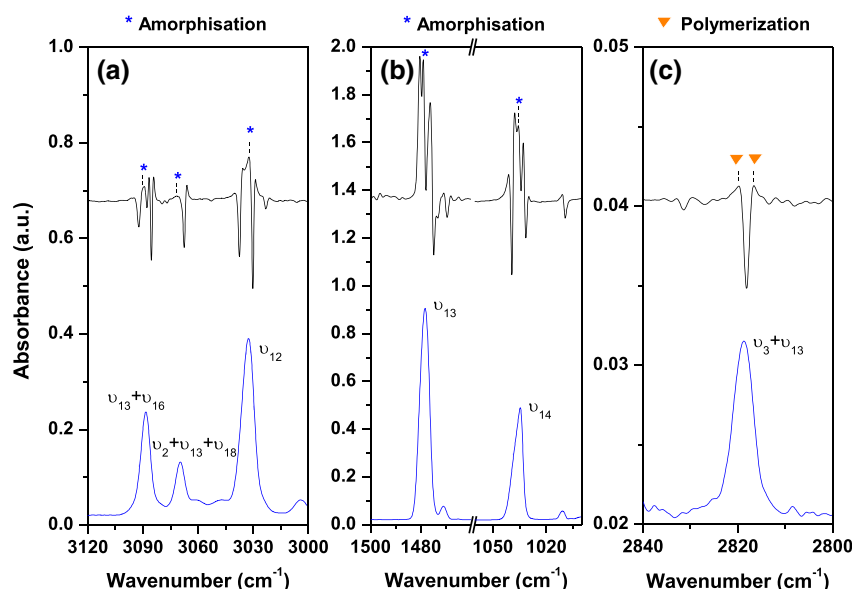
Figure 6. Comparison of the subtraction FTIR spectrum (after-before UV irradiation) of case 1 benzene ice at 70 K (top), with the infrared spectrum of amorphous benzene ice at 50 K (bottom), in different spectral regions (a) between 3,120 and 3,000\text{ cm}^{-1} , (b) between 1,500 and 1,000\text{ cm}^{-1} , (c) between 2,840 and 2,800\text{ cm}^{-1} . Peaks marked with asterisks correspond to amorphous benzene features while features characteristic of polymerization are marked with triangles.
