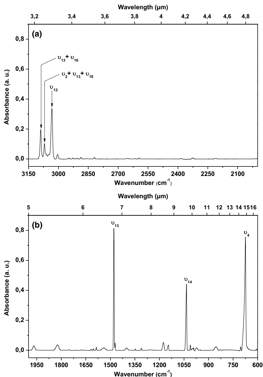
Figure 1. Infrared spectrum of amorphous benzene (deposited 16 K) in two regions: (a) between 3,150 and 2,025 cm -1 and (b) between 1,975 and 600 cm -1 ; small bands on the spectrum correspond to harmonics or combination modes.
