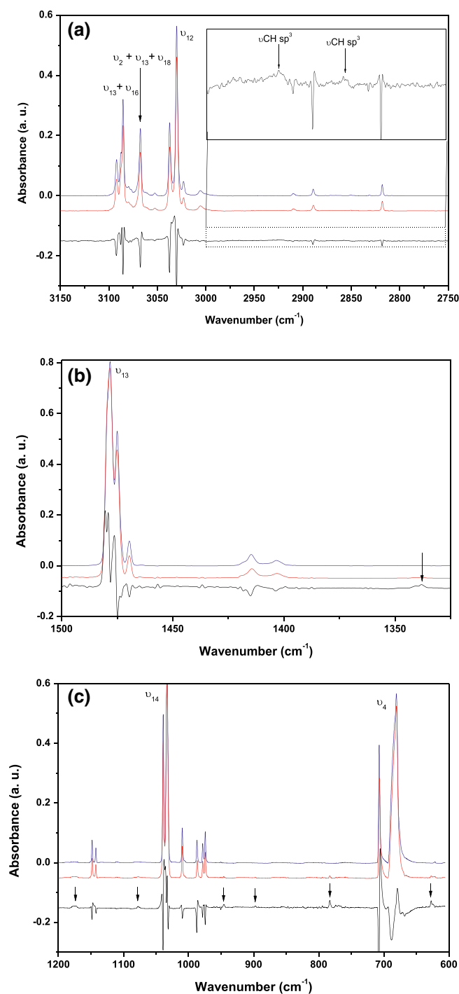
Figure 4. FTIR spectra of C_6H_6 at 70 K (case 1), presented in different areas (a) between 3,150 and 2,750 cm^{-1} , (b) between 1,500 and 1,300 cm^{-1} , (c) between 1,200 and 600 cm^{-1} : (blue)/(red) before/after 2,880 min of irradiation ( \lambda > 230 nm) and (black) subtraction spectrum multiplied by a factor of 3. Arrows highlight the new photo-produced spectral features corresponding to the fulvene isomer. For the interpretation of the legend, the reader must refer to the web version of this article.
