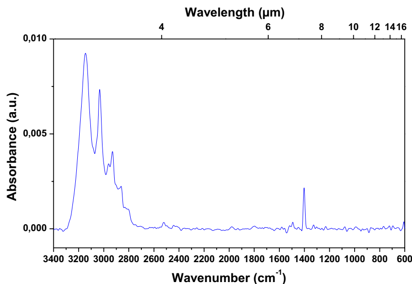
Figure 8. FTIR spectra recorded at 300 K of the residue produced by UV radiations ( \lambda > 230 nm) of C_6H_6 ice at 70 K followed by a warm-up to 300 K.
