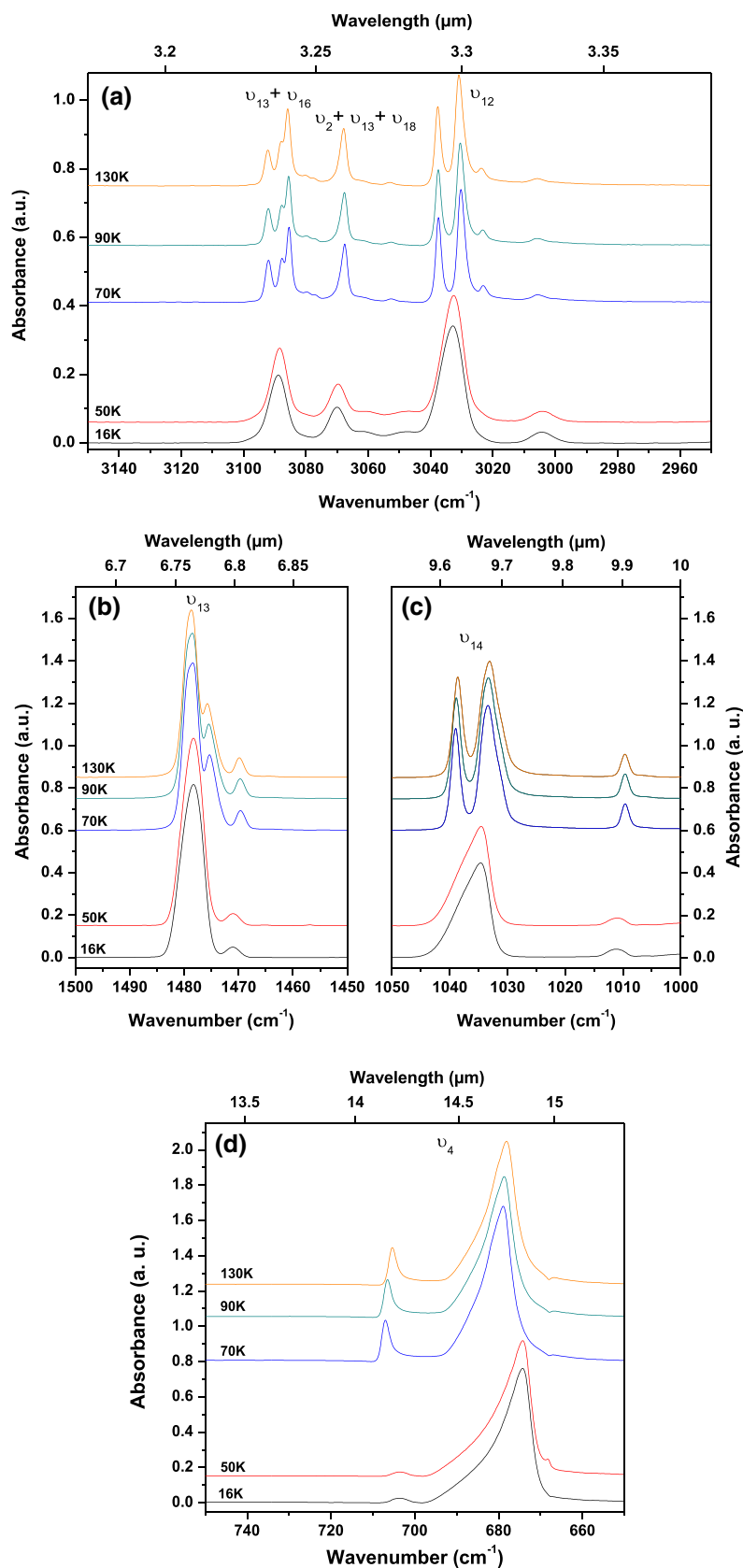
Figure 3. Infrared spectra of \text{C}_6\text{H}_6 (amorphous ice) (16 K and 50 K) and (crystalline ice) (70 K, 90 K, and 130 K) in different areas labeled (a–d) characteristics of the most intense bands of the benzene ice.
