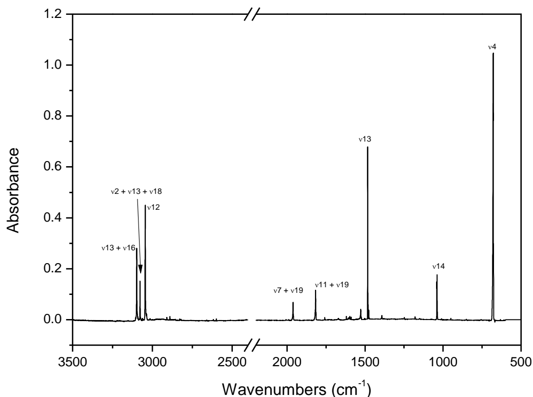
130 131 Figure 1: Infrared spectrum of benzene trapped in nitrogen matrix at 14 K. The spectrum 132 has been truncated in the middle in order to omit the gaseous CO 2 133
