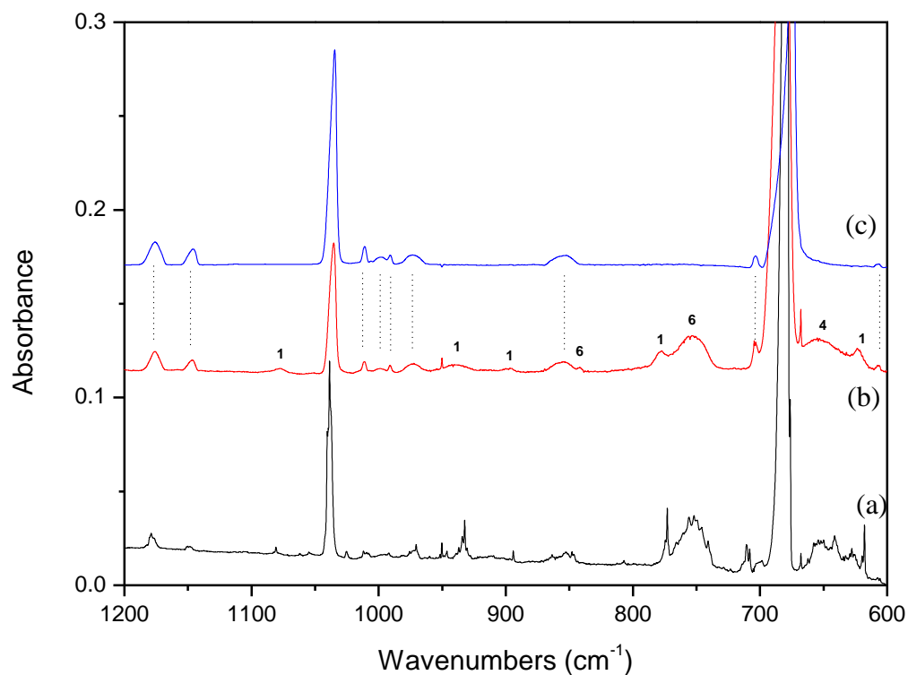
Figure 5: Infrared spectra recorded during the warming-up performed at the end of the photolysis experiment ( \lambda > 230 nm) of benzene trapped in N 2 matrix: (a) at 14 K after 30K, (b) at 40 K after N 2 sublimation (c) benzene ice at 40K 1:fulvene. 4: substituted acetylene. 5: acetylene. 6: substituted benzene.
