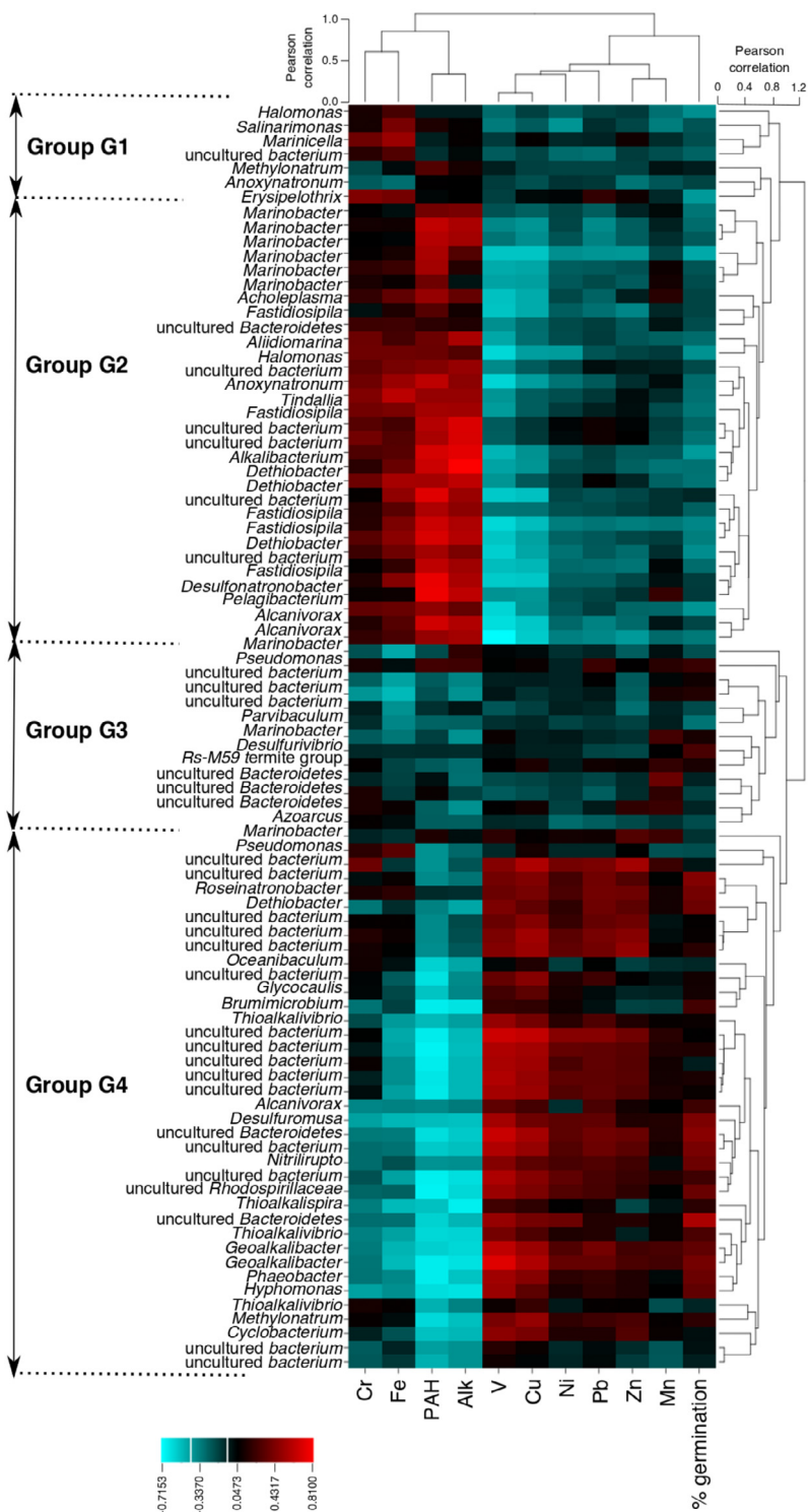
Fig. 4. Clustered correlation (ClusCor) between bacterial OTU abundances and pollutant (metals and hydrocarbons) contents, and wheat germination. Clustering was performed applying Pearson correlations and Ward algorithm, red indicating high positive correlation and blue high negative correlation ( p value < 0.01). The analysis was performed at the OTU level, with 100 most abundant OTUs, applying a threshold similarity of 97% for OTU identification. Biological replicates ( n = 3 ) were used. (For interpretation of the references to colour in this figure legend, the reader is referred to the web version of this article.)
