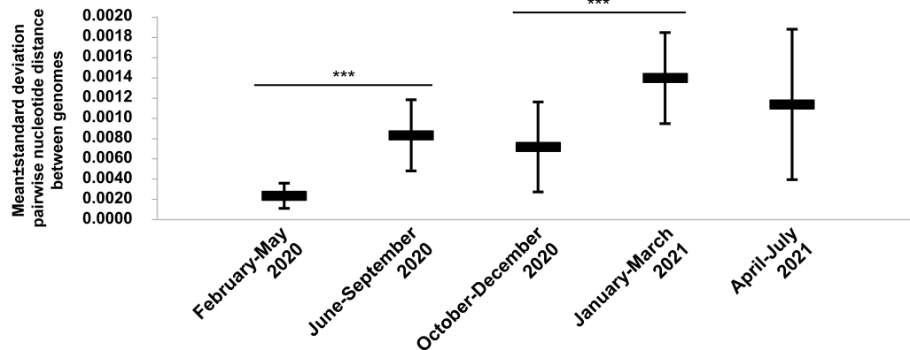
FIGURE 3 | Chronological distribution of mean ( \pm standard deviation) pairwise genetic distances according to time periods for SARS-CoV-2 genomes obtained from patients SARS-CoV-2-diagnosed at IHU Méditerranée Infection, Marseille. *** p < 10^{-3} .
