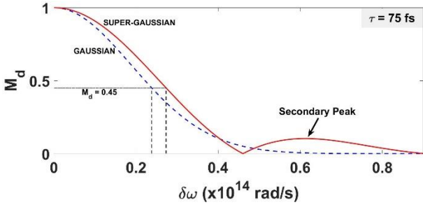
Figure 5. M_d vs \delta_\omega for Gaussian beams and super-Gaussian beams at \tau = 75 fs.
