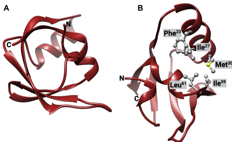
Figure 3. Crystal structure of BfFeoA . A, similar to other FeoA proteins structurally characterized, BfFeoA adopts an SH3-like fold, which is characterized by a small \beta -barrel. B, like observed in the structure of KpFeoA (PDB ID 6E55), BfFeoA contains a “C-shaped” clamp region lined with hydrophobic residues (shown in ball and stick), composed of Phe 23 , Ile 27 , Met 30 , Ile 59 , and Leu 61 . This view represents a 100^\circ rotation about the y-axis and a 40^\circ rotation about the x-axis of panel A. Labels 'N' and 'C' refer to the N- and C-termini, respectively. Figure created with BioRender.
