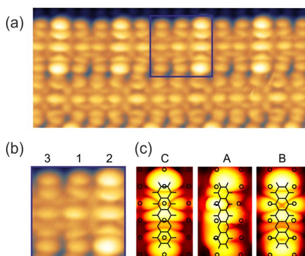
Fig. 3 (a) Experimental STM images of DHTAP molecules forming chains of the (7:9) HOC phase. (b) Zoom into the area highlighted in (a), depicting three neighbouring molecules in different registry with the substrate. (c) Simulated STM images based on the DFT calculations for a single DHTAP molecule in configuration C, A and B in Fig. 2(a), respectively.
