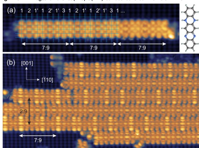
Fig. 1 STM images of the Cu(110)-O(2×1) surface covered with 0.5 ML of DHTAP.
