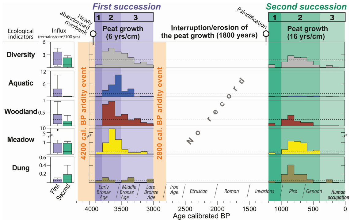
Figure 4. Long-term ecological successions of the Mediterranean wetland of Bagliettu evidenced by a selection of meaningful insect-inferred indicators influxes (that is, diversity, aquatic, woodland, meadow, dung) that are represented by step-curves according to a constant time-interval of 100 years. Three phases of ecological successions (phase 1: waterlogging and early stage of organic deposition, phase 2: abundant and diversified insect assemblages; phase 3: persistence of the former groups, but poorer) are highlighted in a gradient of purple (first succession) and green bands (second succession), interrupted by a recession phase (hiatus or erosion) represented in light grey. The boxplots sum up the individual distributions of the two successions. The dashed line displays the median influx values of the first succession. Two regionally recognized climate aridity event are shown in orange. An indicative chronology of the human occupation and rulership of Corsica is shown.
