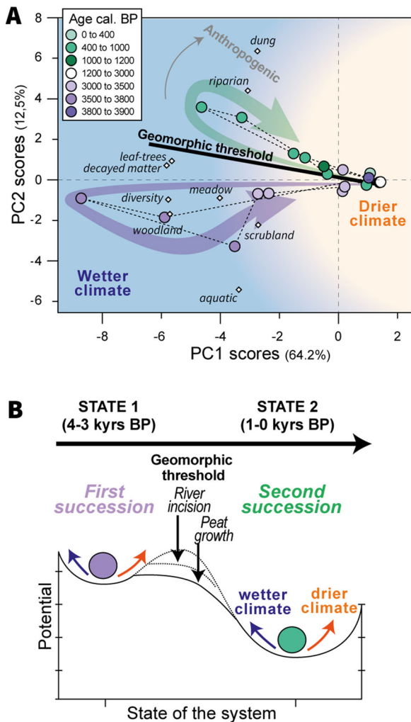
Figure 5. Interpretation of the millennial-long ecological functioning of the Mediterranean wetland of Bagliettu. A Principal Component Analysis (Components 1 and 2) carried out on the homogenized dataset of 39 individuals representing 100 years interval each [circles], and 9 ecologically meaningful variables [diamonds]. The individuals are grouped by phases of successional stage (gradients of purple and green). The dashed lines connect the individuals according to time. A visual guide of interpretation includes the two succession pathways of the peat-bogs (purple and green thick arrows) during relatively wetter climate (blue area), going back to a similar null position in the oriented space, that has been synchronic with drier climate (orange area). A rotation of the individuals toward drier peat conditions is interpreted by the occurrence of the geomorphic threshold (thick black line). Propensity of higher anthropogenic disturbances in the recent time suggests the potential occurrence of a second ecological threshold (light grey). B Schematic representation of the geomorphic-induced regime shift that, by amplifying impacts of climate aridification, has precipitated, 3000 years ago, the wetland ecological functioning to a new, different regime of variability.
