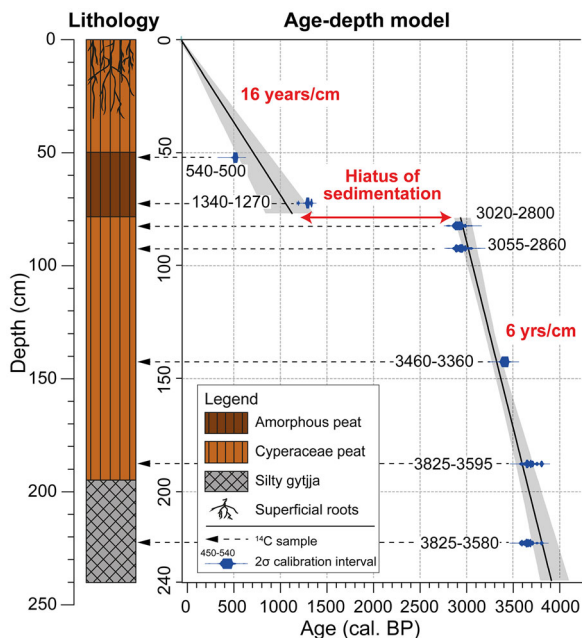
Figure 2. Lithology and age-depth model of the sedimentary profile of Bagliettu computed based on the probability density functions of the ^{14}\text{C} AMS ages. The bold line represents the best age-depth model solution and the grey envelope with the 95% confidence interval.
