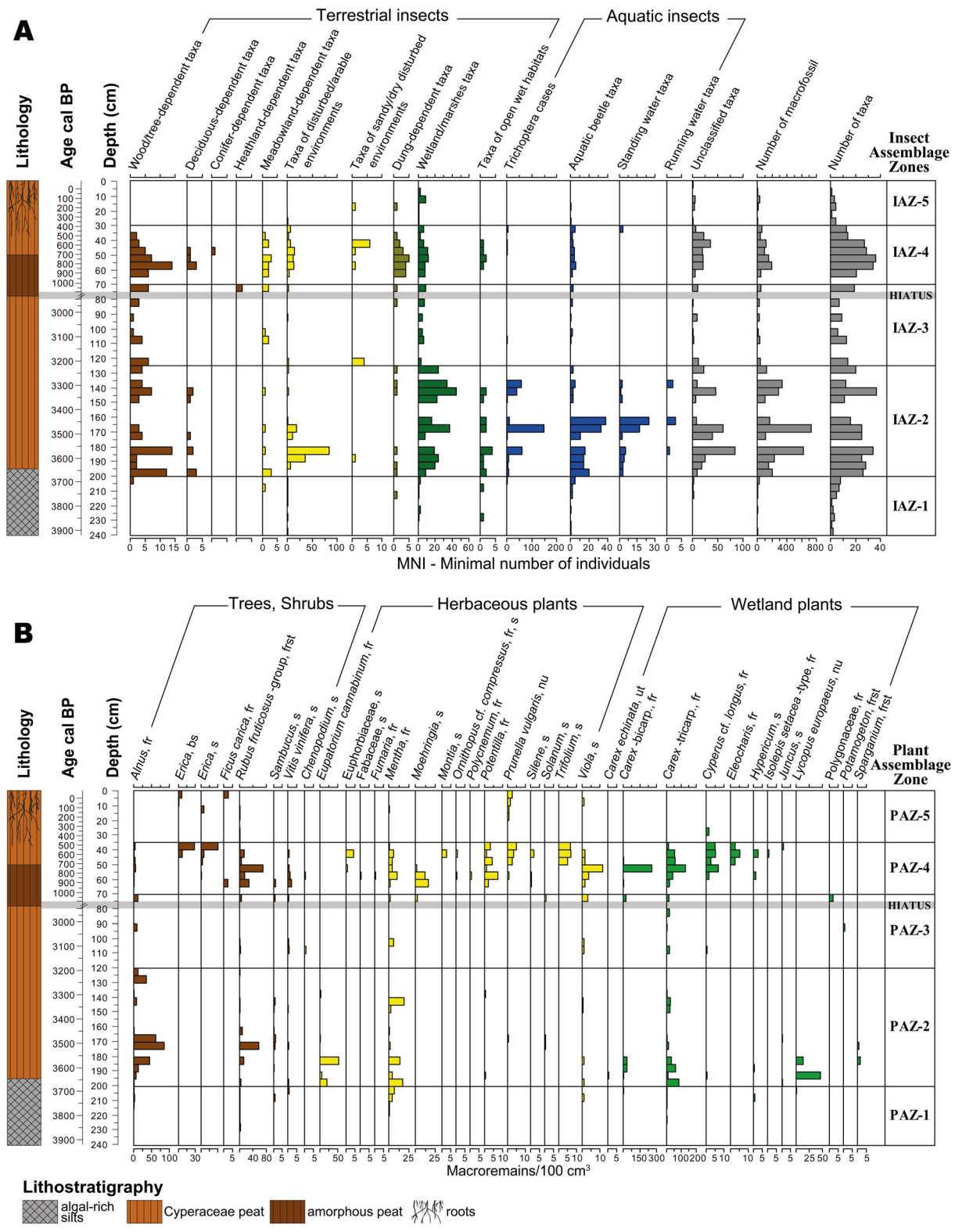
Figure 3. Fossil remains identified in the sediments of the wetland of Bagliettu represented according to the core depth (cm) and the corresponding best-modelled age (years calibrated Before Present). The horizontal grey band symbolizes a sedimentary hiatus. A Simplified entomological diagram expressed as Minimum Number of Individuals (MNI) per sample. IAZ: Insect Assemblage Zone. B Plant macrofossils diagram expressed in concentration (number of macro remains per 100 cm 3 ). Fr fruit, s seed, bs buds, frst fruitstone, nu nutlets, ut utricle. PAZ plant assemblage zone.
