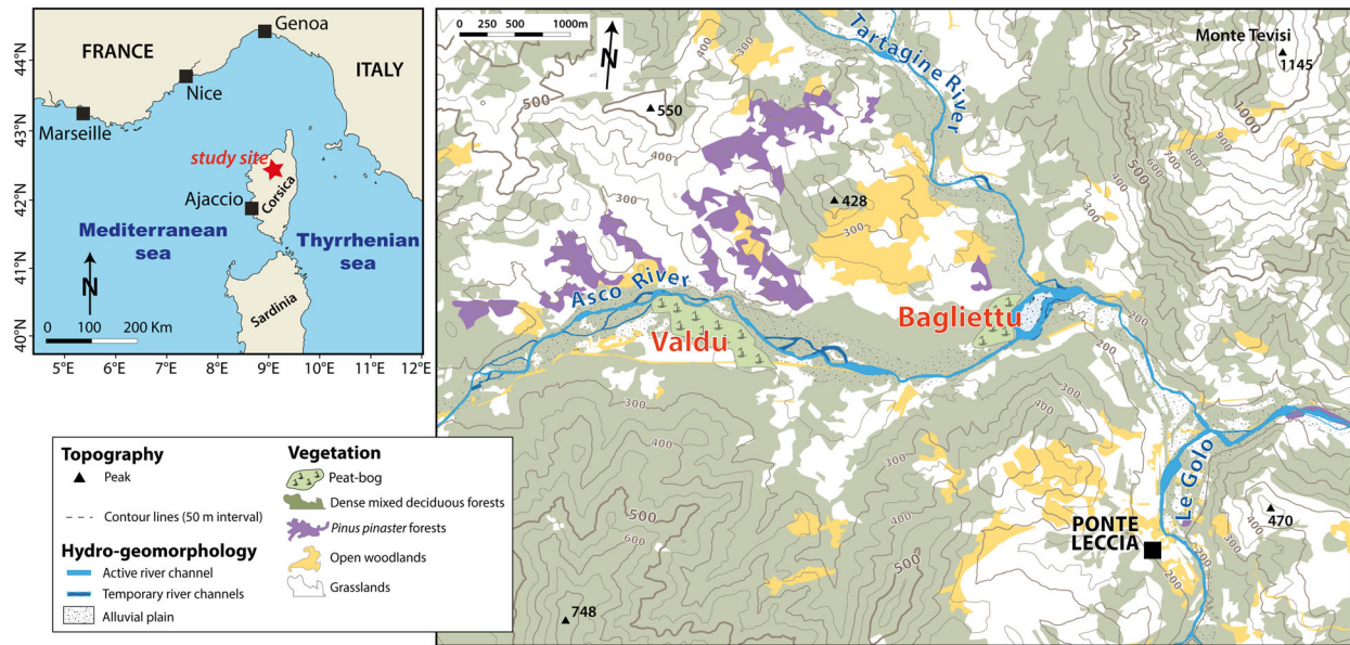
Figure 1. Location map of the study site, in the sub-humid dry Mediterranean region. The wetland of Bagliettu is situated on the left bank mountain river of Asco, perched at 1.5 m above the active channel, at 210 m a.s.l. The area is situated in the meso-Mediterranean vegetation stage dominated by a mixed deciduous forest on the north-facing slopes while south-exposed flanks are covered by xeric shrub and grasslands.
