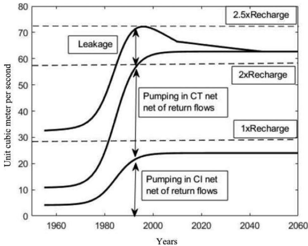
Fig. 8 Global water balance of the NWSAS
