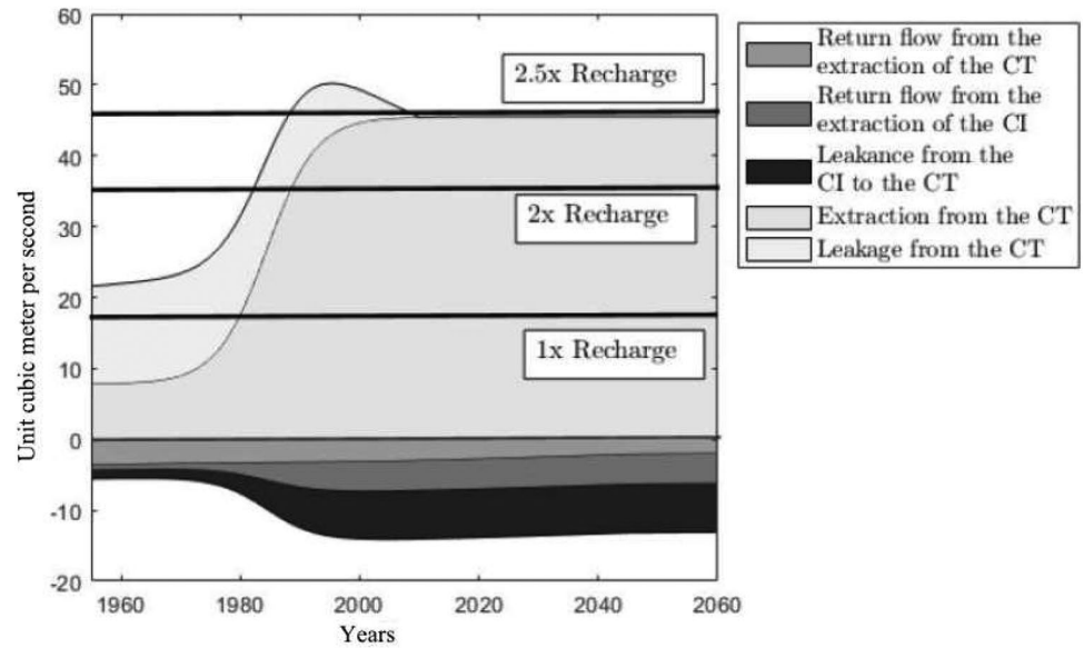
Fig. 10 Water balance of the CT
