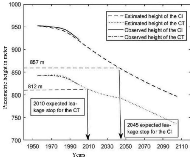
Fig. 5 Evolution of the piezometric levels in the NWSAS
