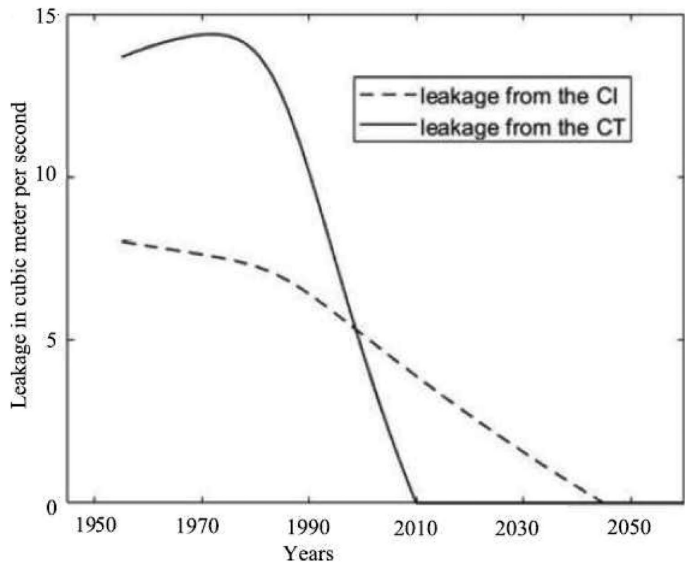
Fig. 6 Evolution of the leakages
