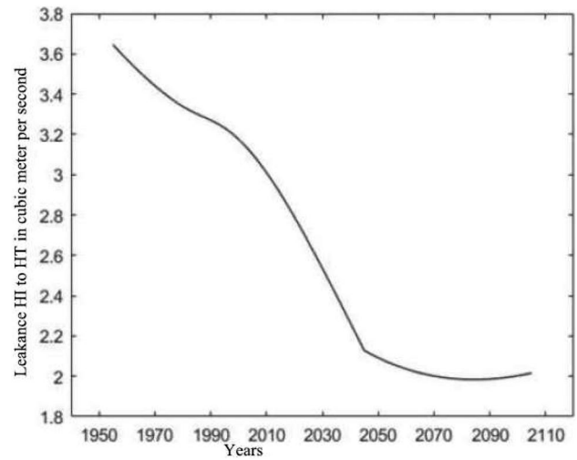
Fig. 7 Evolution of the leakage from the CI to the CT
