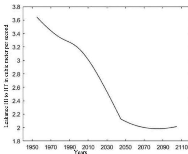
Fig. 7 Evolution of the leakance from the CI to the CT
