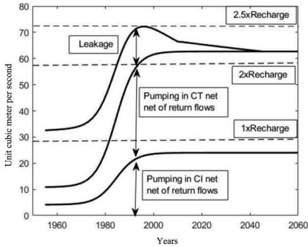
Fig. 8 Global water balance of the NWSAS
