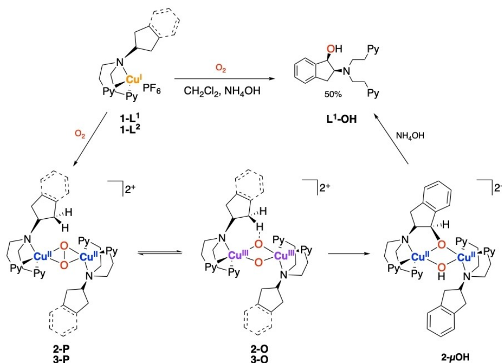
Scheme 2. Schematic representation of the possible intermediate species in the hydroxylation reaction of L^1 and L^2 starting from mononuclear 1-L^1 and 1-L^2 , respectively. Note that hydroxylation is not observed experimentally in the case of L^2 .
