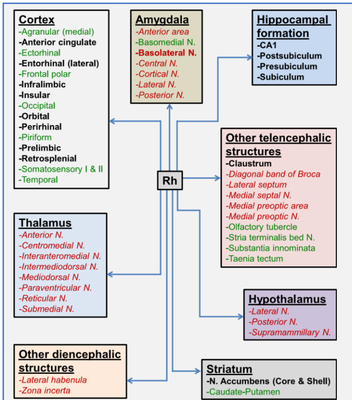
Fig. 4. Brain regions innervated by the rhomboid (Rh) nucleus. The regions indicated in bold (black) receive dense projections from the Rh nucleus. The regions in italics (red) are sparsely innervated. Those printed in normal type (green) receive intermediate innervation densities. Abbreviation: N. stands for nucleus or nuclei. According to Dolleman-Van der Weel and Witter (1996); Vertes et al. (2006, 2007, 2010), and to Cholvin (2014, PhD thesis), from which this figure was inspired.
