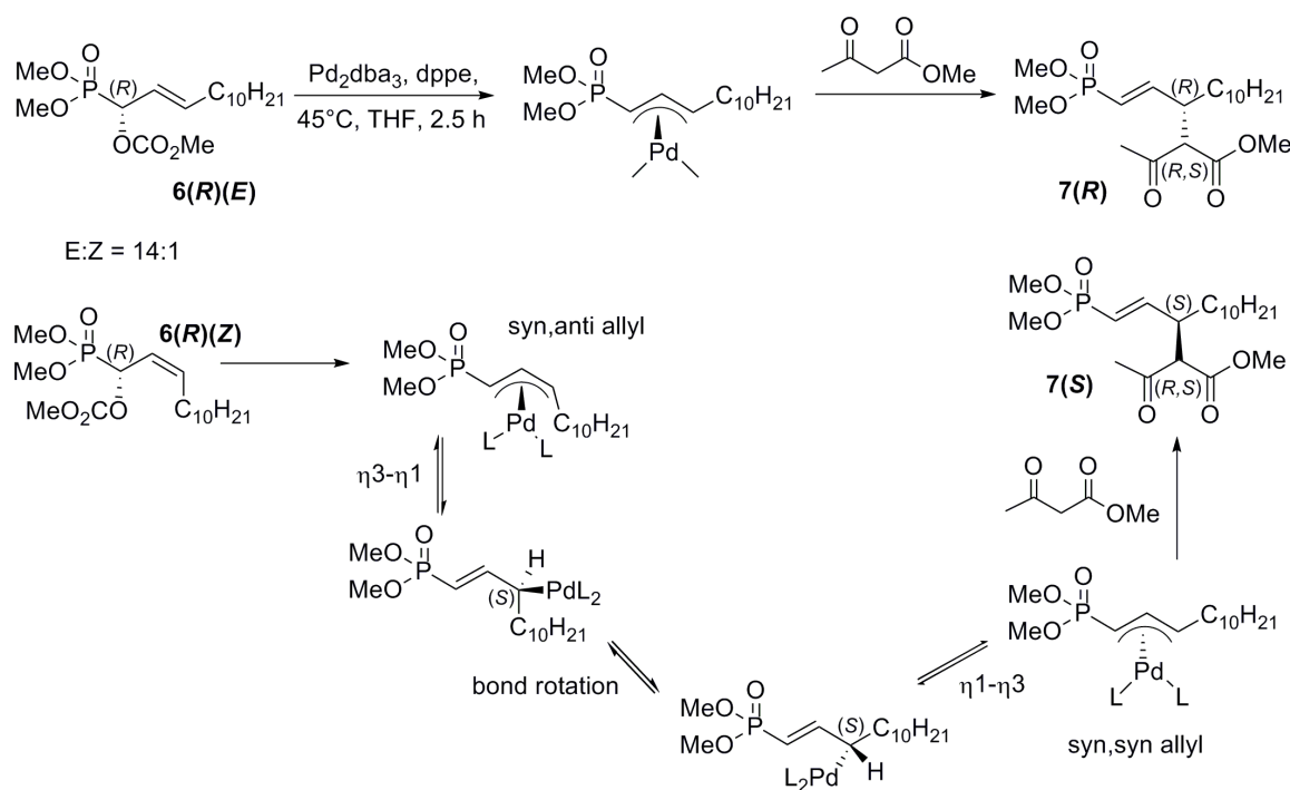
Scheme 3. Mechanism for the palladium(0)-catalyzed reaction of 6(R)(E) and 6(R)(Z) with methyl acetoacetate. 27
