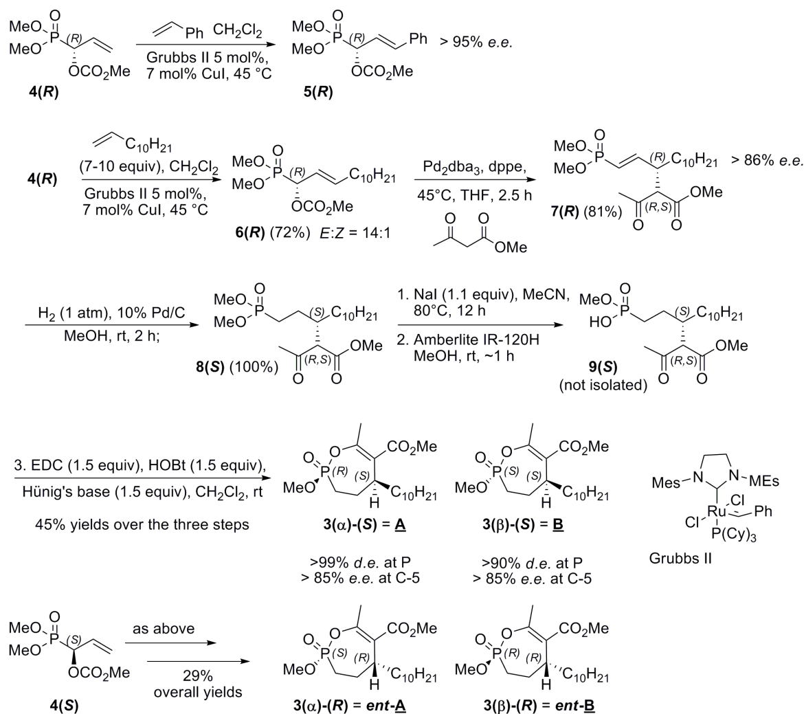
Scheme 2. Asymmetric synthesis of the diastereoisomers of the monocyclic enolphosphonates 3(α) and 3(β) .
