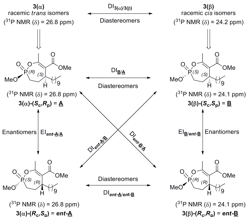
Scheme 4. Stereochemical relationships between the four monocyclic enolphosphonate isomers 3 analogous to Cyclophostin.
