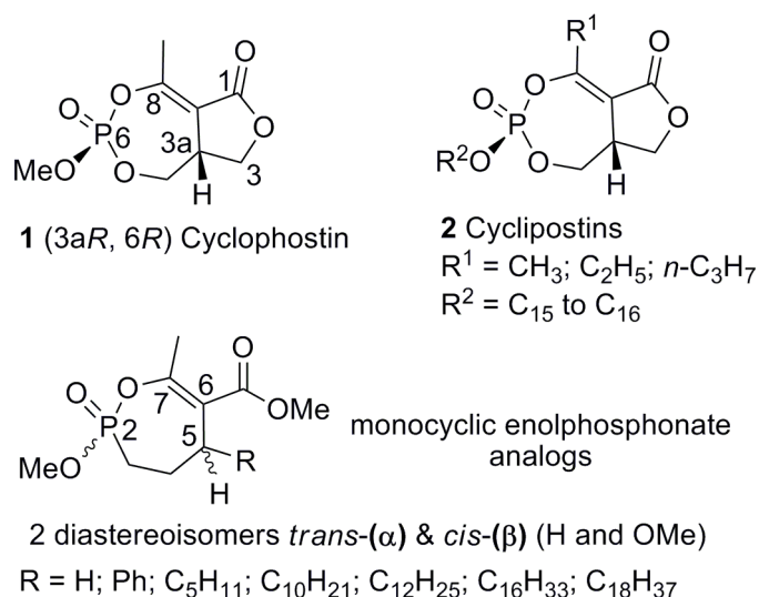
Scheme 1. Structure of Cyclophostin 1 , Cyclipostins 2 and related enolphosphonate analogs 5 recently reported.
