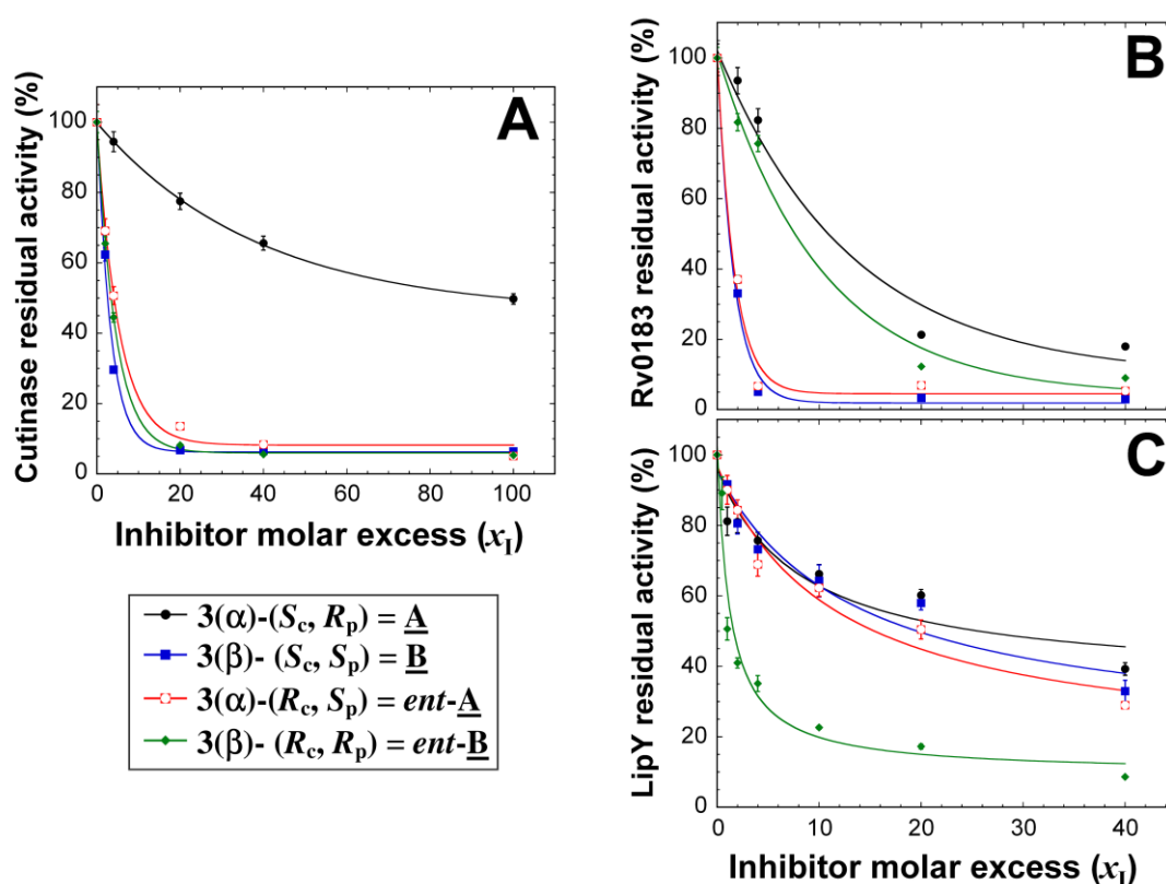
Figure 1: Variation of the residual activities of (A) Cutinase, (B) Rv0183 and (C) LipY as a function of increasing molar excess ( x_1 ) of compounds 3 ( \alpha )-( S_c , R_p ) ( \bullet ), 3 ( \beta )-( S_c , S_p ) ( \blacksquare ), 3 ( \alpha )-( R_c , S_p ) ( \square ) and 3 ( \beta )-( R_c , R_p ) ( \blacklozenge ). Each enzyme was pre-incubated at various inhibitor molar excess for 30 min at 25 °C. Kinetic assays were performed as described in Experimental Section . Results are expressed as mean values \pm standard deviation of at least three independent assays (CV% < 5.0%).
