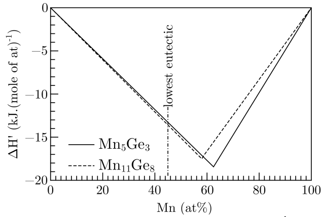
Figure 2: The effective heats of formation \Delta H' of the phases Mn_5Ge_3 and Mn_{11}Ge_8 versus the Mn concentration.
