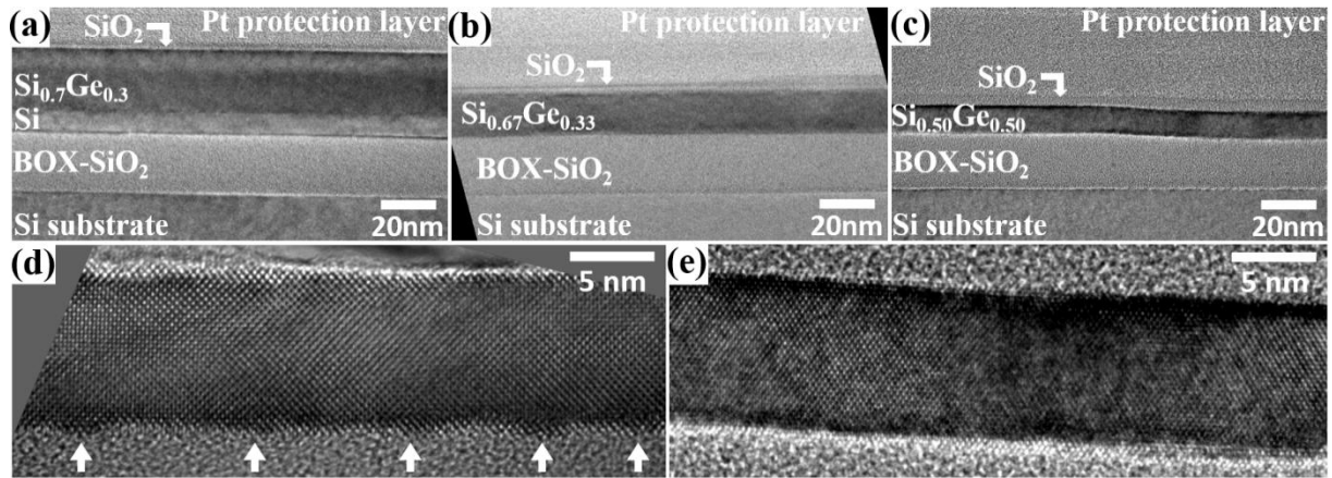
Figure 6: TEM cross-section images (along the [110] crystallographic axis) of the samples A (initial structure) (a), B (oxidized during 120min) (b) and C (oxidized during 300min) (c) where the stacking layers are well visible: Si substrate/20nm BOX/8nm SOI/ \text{Si}_{1-x}\text{Ge}_x layer and top \text{SiO}_2 layer for samples B and C. HRTEM of sample C: (d) arrows indicate the protrusions; (e) small rotation of the crystallographic planes
