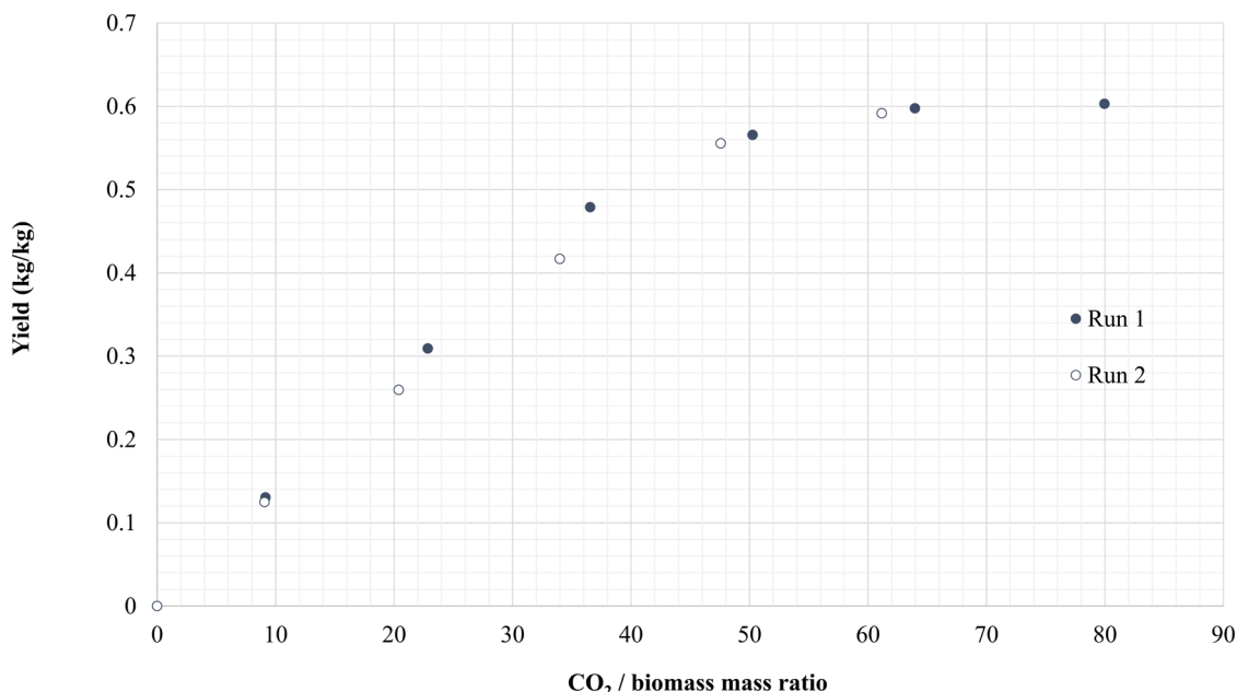
Fig. 3. Repeatability test perform at 400 bar, 333 K and 0.18 kg/h.
