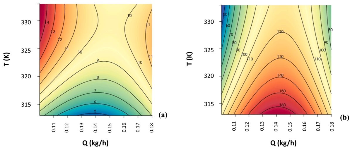
Fig. 5. Surface plot of (a) Argan oil apparent solubility (g oil /kg CO2 ) in SC-CO 2 and (b) the CO 2 /biomass mass ratio (kg CO2 /kg biomass ) for reaching a yield of 60% as function of flow rate and temperature.
