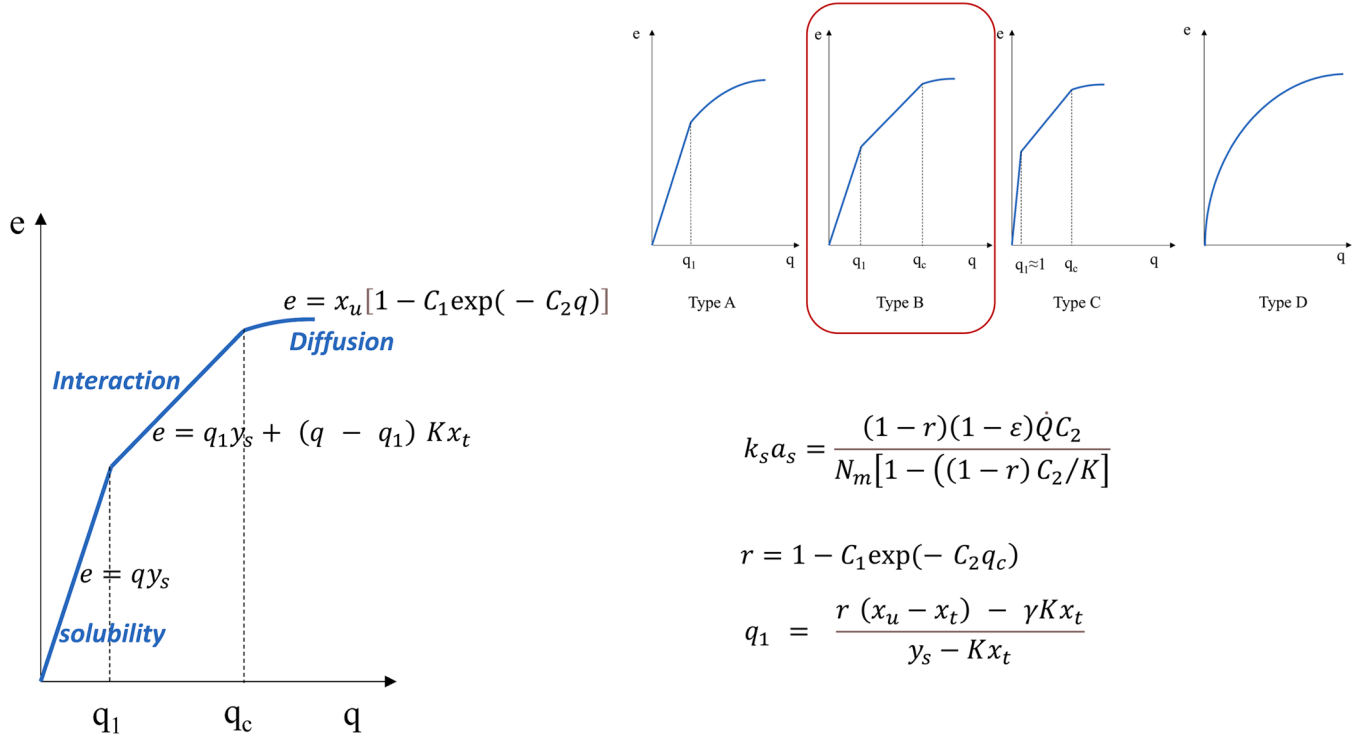
Fig. 2. Type of extraction in Sovová's BIC model.
