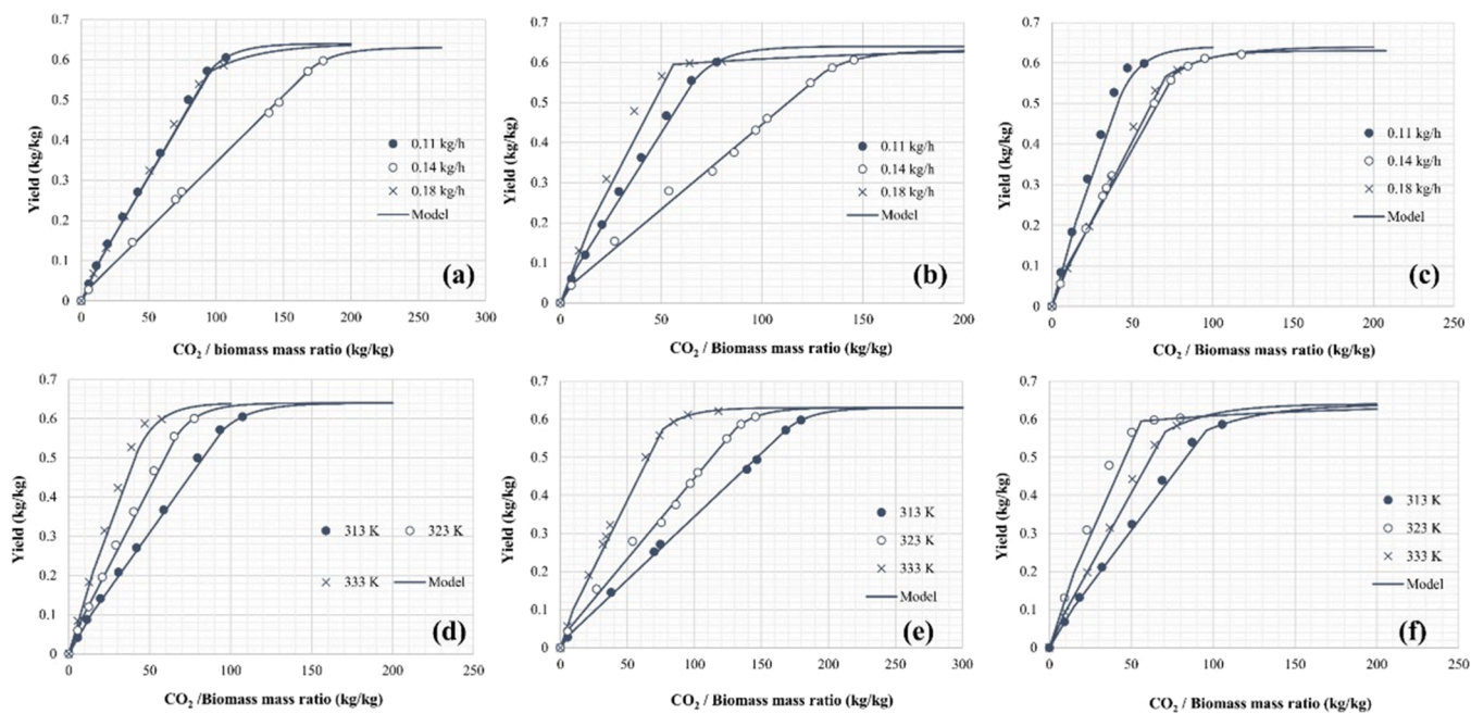
Fig. 6. SC-CO 2 extraction kinetics at 400 bar and (a) 313 K, (b) 323 K, (c) 333 K, at CO 2 flow rate of (d) 0.11 kg/h, (e) 0.14 kg/h and (f) 0.18 kg/h.
