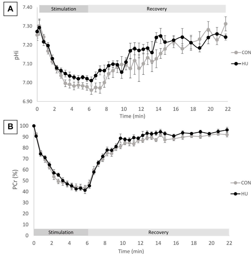
FIGURE 1 | (A) pH i time course during the rest-stimulation-recovery protocol in CON and HU. Results are presented as means ± SEM. (B) Relative PCr time-course during the rest-stimulation-recovery protocol in CON and HU. Results are presented as means ± SEM.
