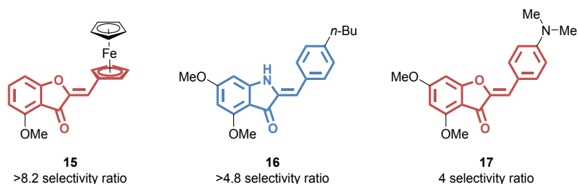
Figure 4. Structures and activities of collateral sensitivity inducers.
