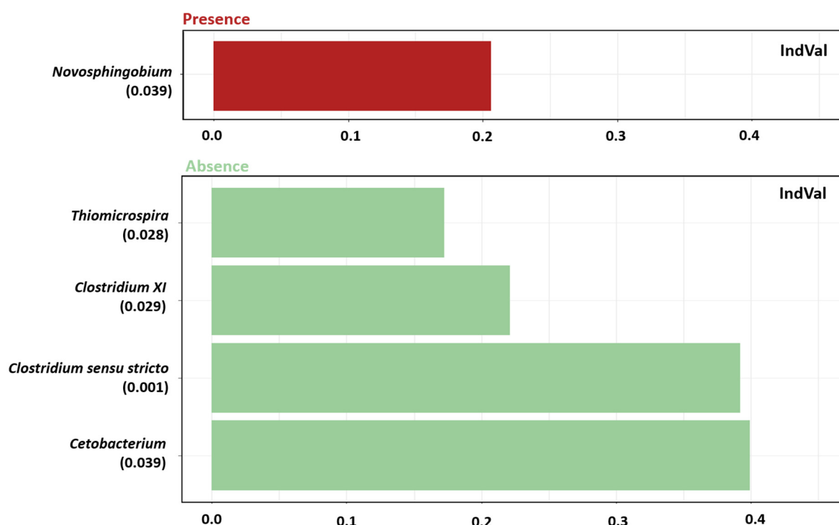
Figure 5. Indicator values of specific bacterial genera of provisioned and non-provisioned sharks; p -values in brackets.
