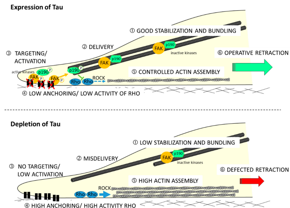
Figure 2. Tau regulates the microtubule-dependent migration of glioblastoma U87MG cells via the Rho-ROCK signaling pathway. Directional cell migration requires spatiotemporal control of focal adhesion formation and dissociation: (upper model) in Tau-expressing cell, good stabilization and bundling of microtubules (1) are positioned at the tail of polarized cells; during migration, the active phosphorylated forms of FAK and p190-RhoGAP proteins are delivered (2) to focal adhesion at the rear of cells (3), thus reducing anchoring and limiting activity of the Rho-ROCK axis (4); this could moderate actin polymerization (5); and good tail retraction results on, which contributes to a coordinated back-to-front movement of cell; (lower schema) in Tau-depleted cells, microtubules are less stabilized and weakly organized in bundles in the back of cells (1); the delivery of FAK and p190-RhoGAP proteins to the back of cells is defected (3); high anchoring on focal adhesion and removal of the restrictive activity of the Rho-ROCK pathways (4) leads to excessive actin polymerization (5); and bad tail retraction is observed.
