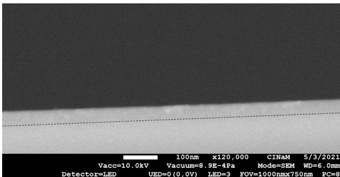
Figure S3. SEM image of a cross-section of the layer \text{M:N}_{10}:\text{OA} spin-coated on a substrate. The 50 nm thick layer is present above the dashed line, and the brighter spots within the layer are attributed to the homogeneously dispersed nanohybrids.
