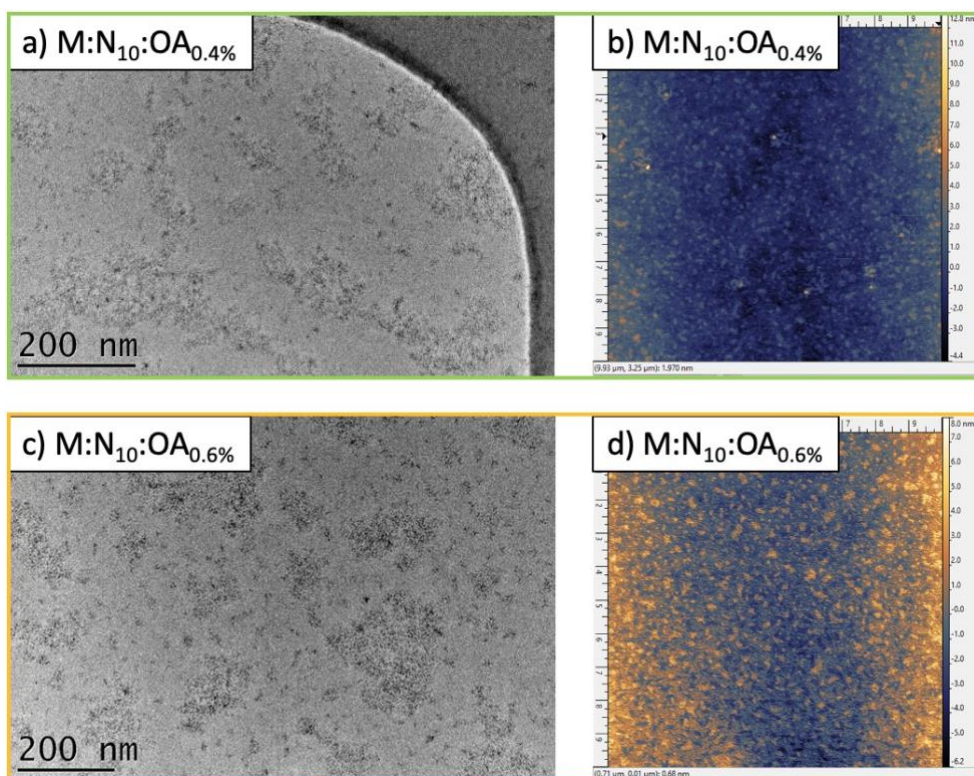
Figure S2. TEM (a) and AFM (b) images of the layer \text{M:N}_{10}:\text{OA}_{0.4\%} . TEM (c) and AFM (d) images of the layer \text{M:N}_{10}:\text{OA}_{0.6\%} .
