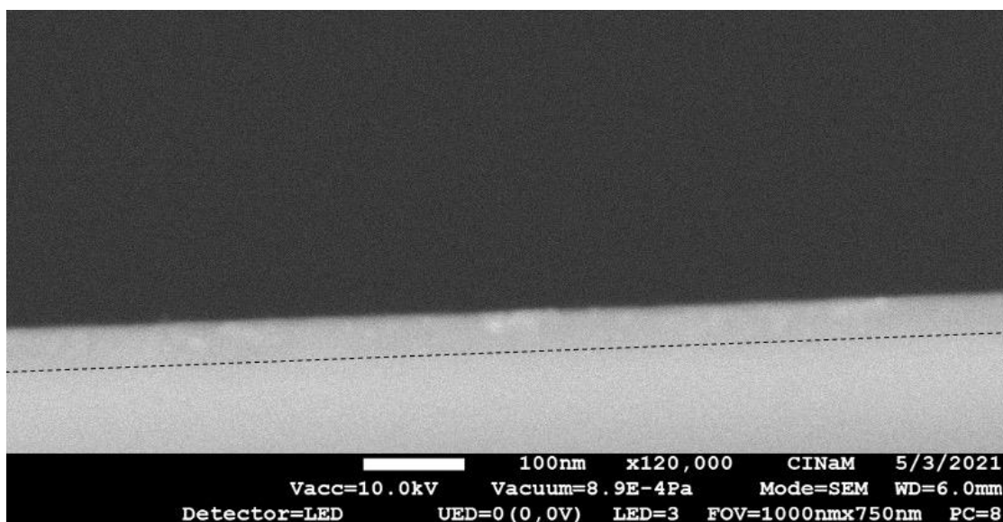
Figure S3. SEM image of a cross-section of the layer M:N 10 :OA spin-coated on a substrate. The 50 nm thick layer is present above the dashed line, and the brighter spots within the layer are attributed to the homogeneously dispersed nanohybrids.
