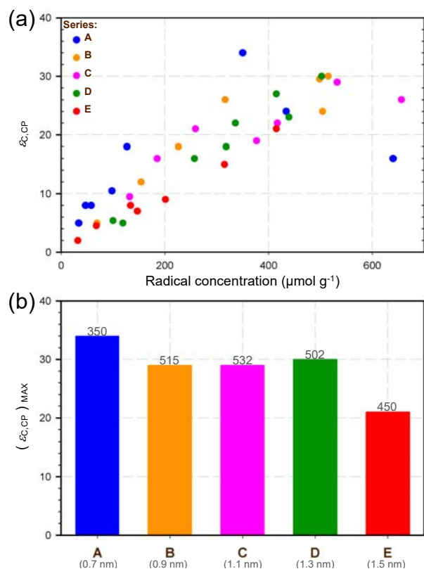
Fig. 3 (a) Evolution of the ^{13}C CP DNP signal enhancement ( \epsilon_{C,CP} ) as a function of the radical concentration for several SBAm-x samples, where x is A, B, C, D, or E (see Fig. 1). \epsilon_{C,CP} was measured on the ^{13}C resonances of a CPMAS spectrum recorded at \sim 105 K on a 0.2 M water solution of U- ^{13}C/^{15}N proline. (b) Maximum \epsilon_{C,CP} value obtained for each of the 5 series of samples considered in this study. The grey numbers reported on top of the coloured bars are the corresponding radical concentrations (expressed in \mu\text{mol g}^{-1} ) whereas those reported below the letters indicate the theoretical distances between the oxygen atoms of the TEMPO rings upon thermolysis.
