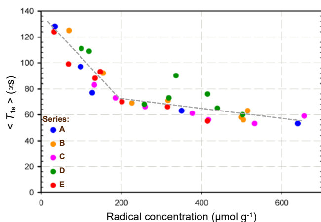
Fig. 4 Evolution of the electron mean recovery time \langle T_{1e} \rangle as a function of the radical concentration for several SBAm-x samples, where x is A, B, C, D, or E (see Fig. 1). \langle T_{1e} \rangle were measured by pulsed EPR at 9.4 GHz on TCE-impregnated samples at 110 K. The dark-grey, short-dashed linear curves of different slopes between 0 and \sim 200 \mu\text{mol g}^{-1} , and between \sim 200 and \sim 600 \mu\text{mol g}^{-1} , respectively, are provided as guides to the eye only.
