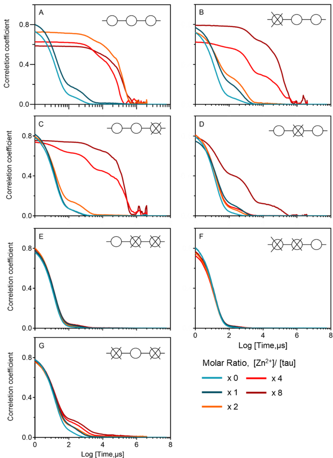
Figure 4. Typical DLS correlation curves of wt-tau and its mutants. 50 \mu M tau in the absence (blue curve) and presence of 50 (dark blue curve), 100 (orange curve), 200 (red curve) and 400 \mu M \text{ZnCl}_2 (brown curve) at 40°C. (A) wt-tau, (B) xoo-tau, (C) oox-tau, (D) oxo-tau, (E) oxx-tau, (F) xxo-tau and (G) xox-tau. For all mutants, experiments were performed at least three times.
