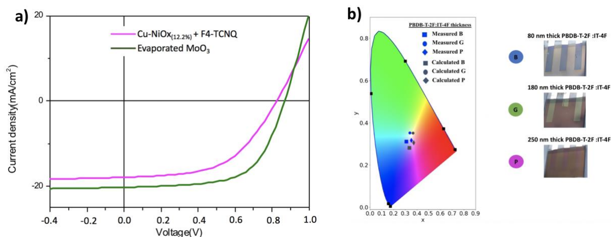
Figure-16: (a) The J–V curves of PBDB-T-2F:IT-4F-based inverted device structures using different HTLs and (b) the color coordinates for the experimental cells (left) along with their photographic images (right). Reproduced from Ref. 134 with permission from the Royal Society of Chemistry.
