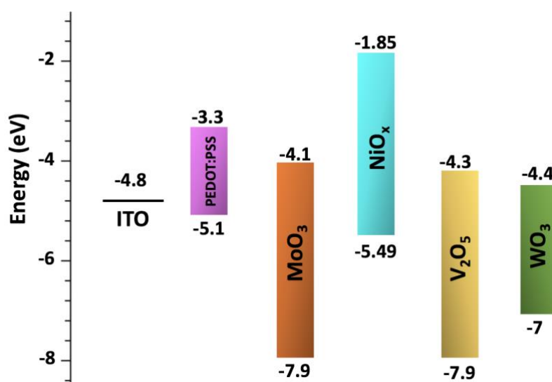
Figure-14: Schematic energy level diagram of typical HTLs used for OSCs.
