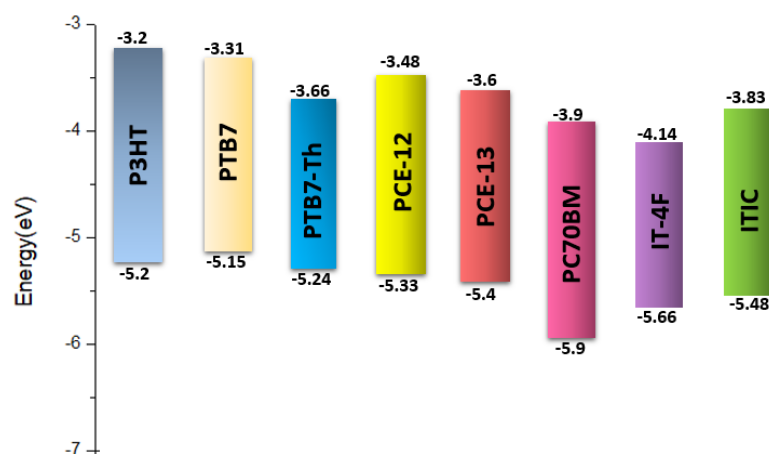
Figure-10: Schematic diagram of the energy levels of some donors and acceptors used for OSCs.
