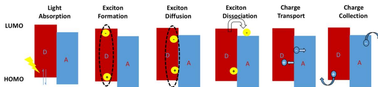
Figure-7: The fundamental steps for the working principle of an OSC.
