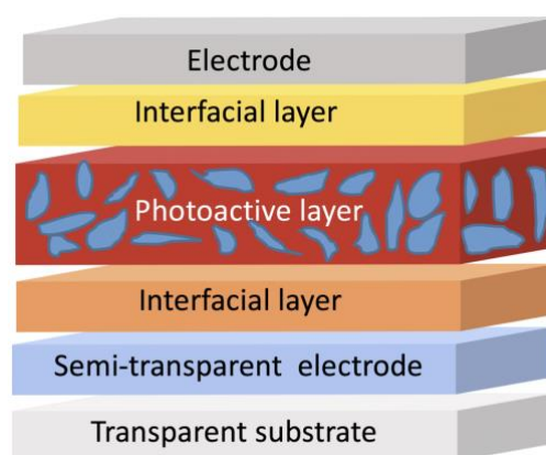
Figure-1: The basic structure of an organic solar cell.
