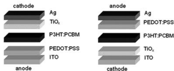
Figure-11: An OSC in the regular (left) and inverted device structure (right).
