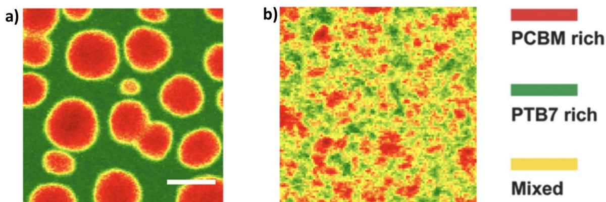
Figure-5: STEM-SI plasmon peak map of PTB7:PC70BM blends processed (a) without DIO and (b) with DIO. Reproduced from Ref. 29 with permission from Wiley Publishing Group.
