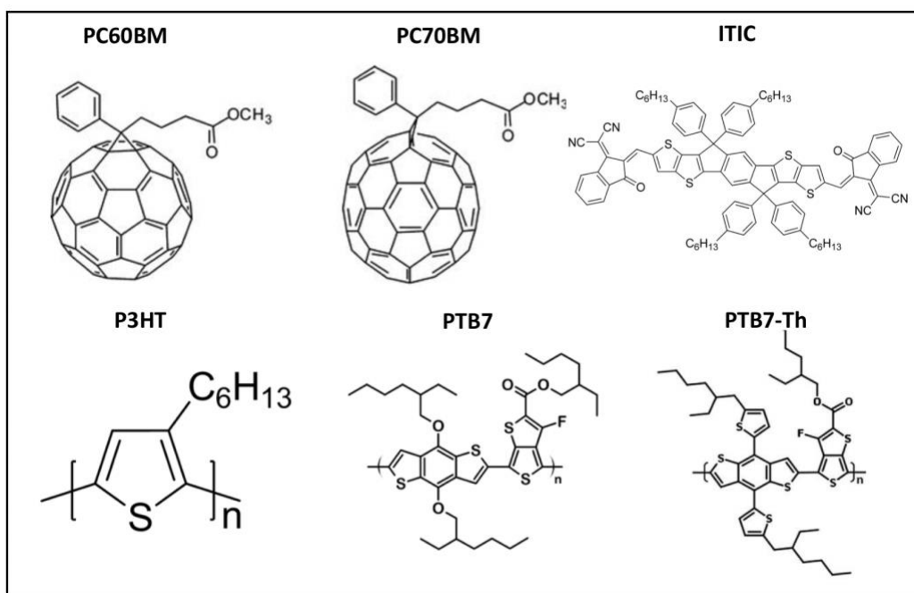
Figure-2: Chemical structures of some donors and acceptors used in OSCs.
