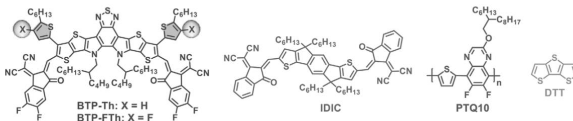
Figure-9: The chemical structures of the NFAs, PTQ10 donor, and DTT additive.
