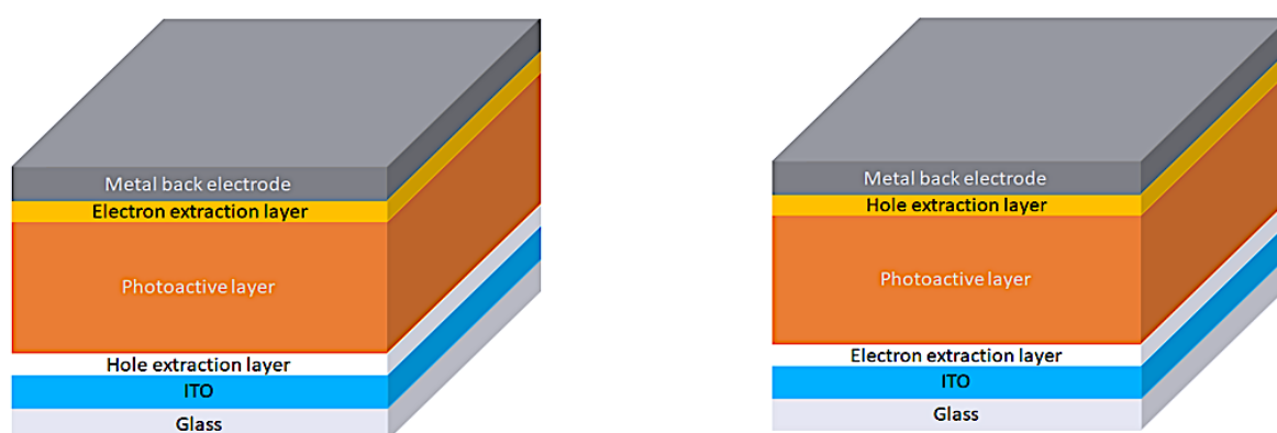
Figure-3: Typical regular (left) and inverted (right) device structures.
